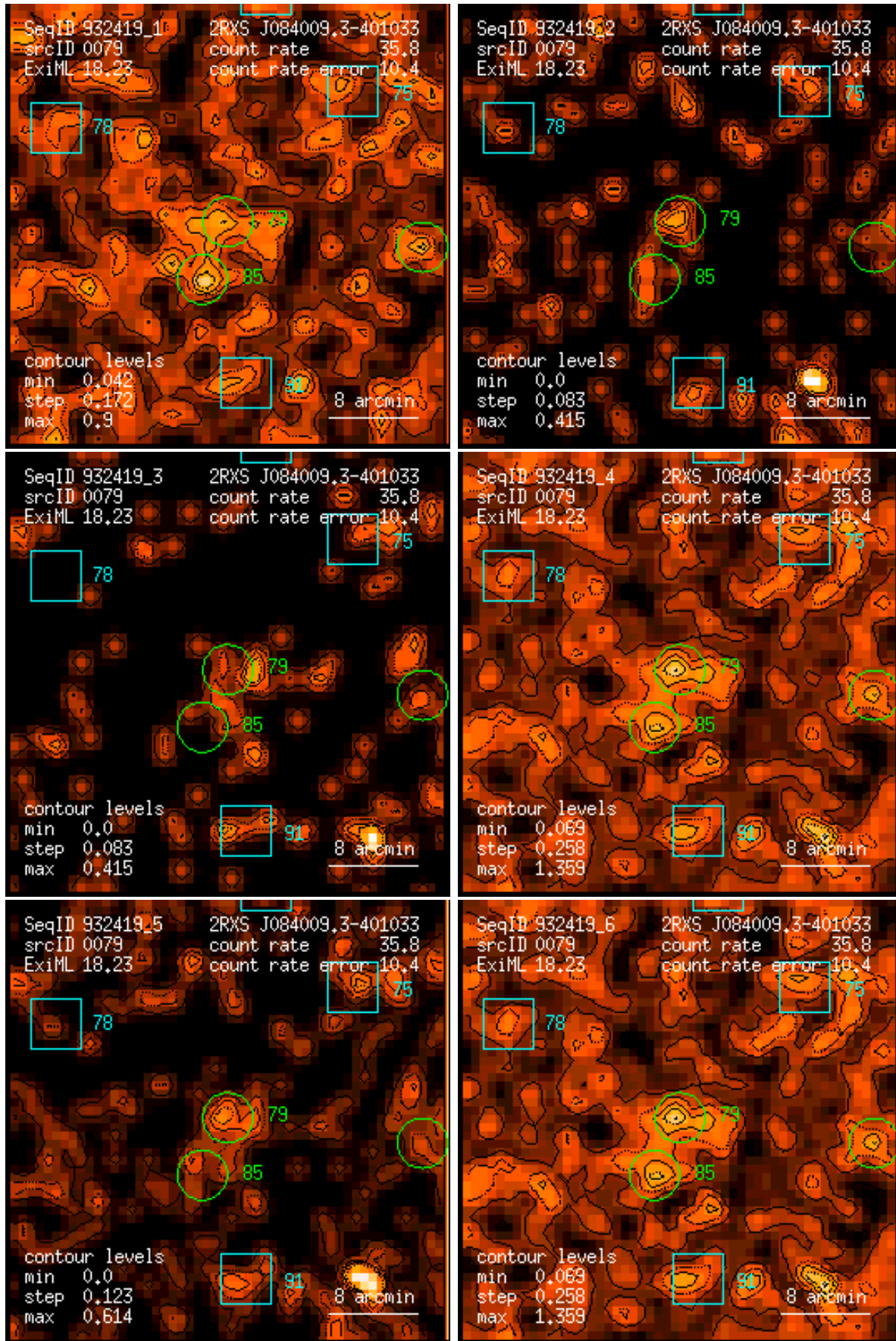
Figure 79: RASS 932419: detection 0079: band rate images, Gaussian filter: (1) PSPC channels 11 – 41, (2) 52 – 90, (3) 91 – 201, (4) 11 – 235, (5) 52 – 201, (6) 11 – 201. Broad band rates in counts/ks. Band rate contour levels in counts/ks/arcmin 2 .
