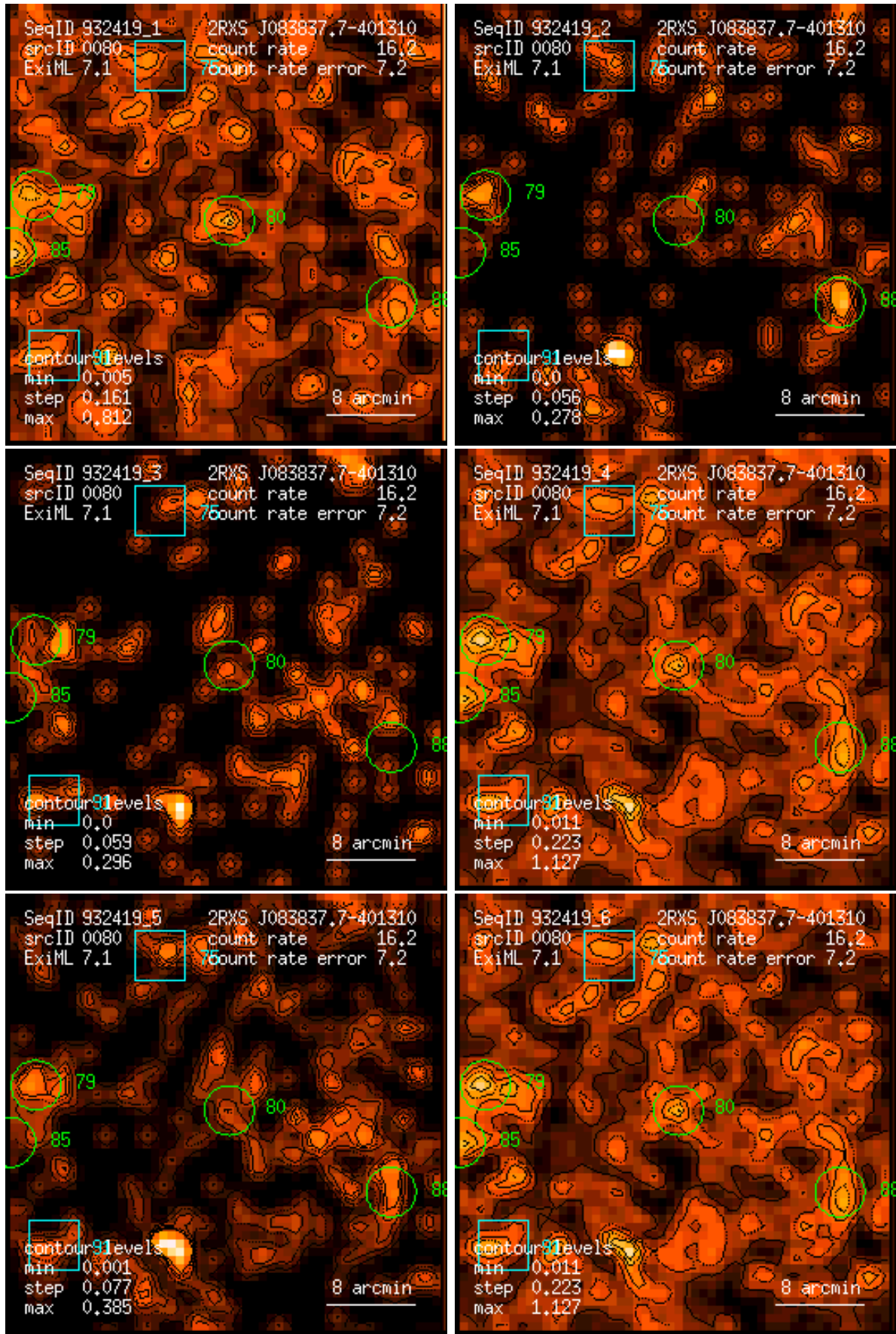
Figure 80: RASS 932419: detection 0080: band rate images, Gaussian filter: (1) PSPC channels 11 – 41, (2) 52 – 90, (3) 91 – 201, (4) 11 – 235, (5) 52 – 201, (6) 11 – 201. Broad band rates in counts/ks. Band rate contour levels in counts/ks/arcmin 2 .
