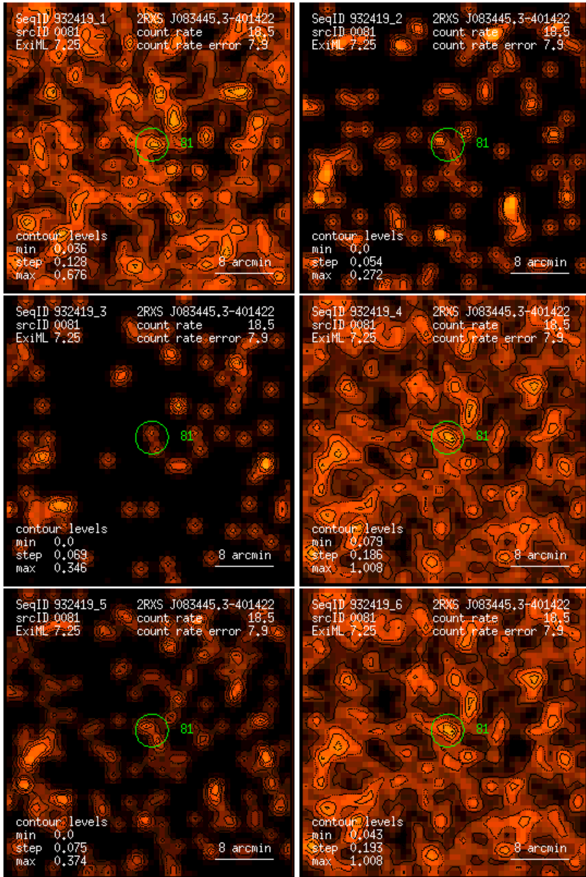
Figure 81: RASS 932419: detection 0081: band rate images, Gaussian filter: (1) PSPC channels 11 – 41, (2) 52 – 90, (3) 91 – 201, (4) 11 – 235, (5) 52 – 201, (6) 11 – 201. Broad band rates in counts/ks. Band rate contour levels in counts/ks/arcmin 2 .
