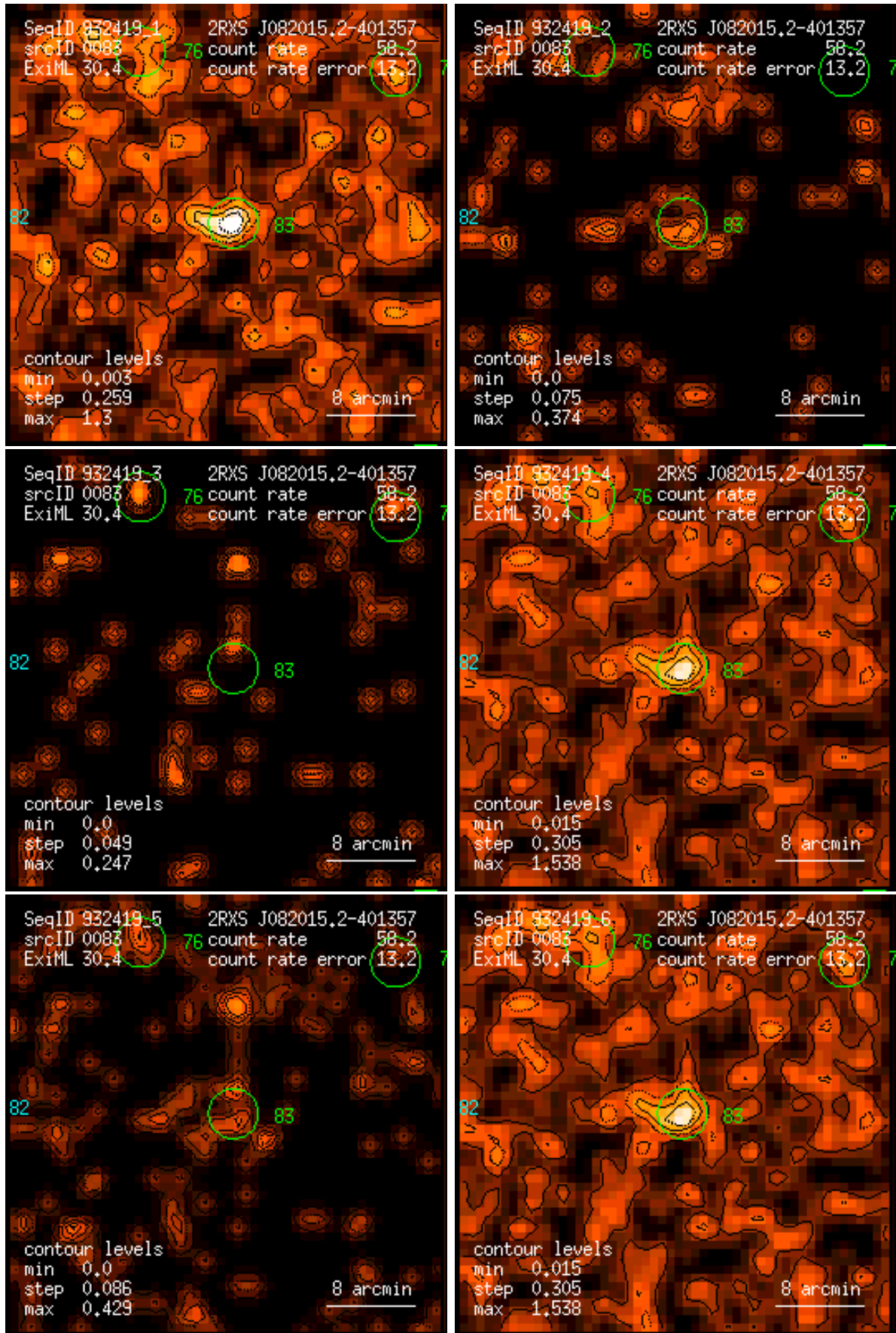
Figure 83: RASS 932419: detection 0083: band rate images, Gaussian filter: (1) PSPC channels 11 – 41, (2) 52 – 90, (3) 91 – 201, (4) 11 – 235, (5) 52 – 201, (6) 11 – 201. Broad band rates in counts/ks. Band rate contour levels in counts/ks/arcmin 2 .
