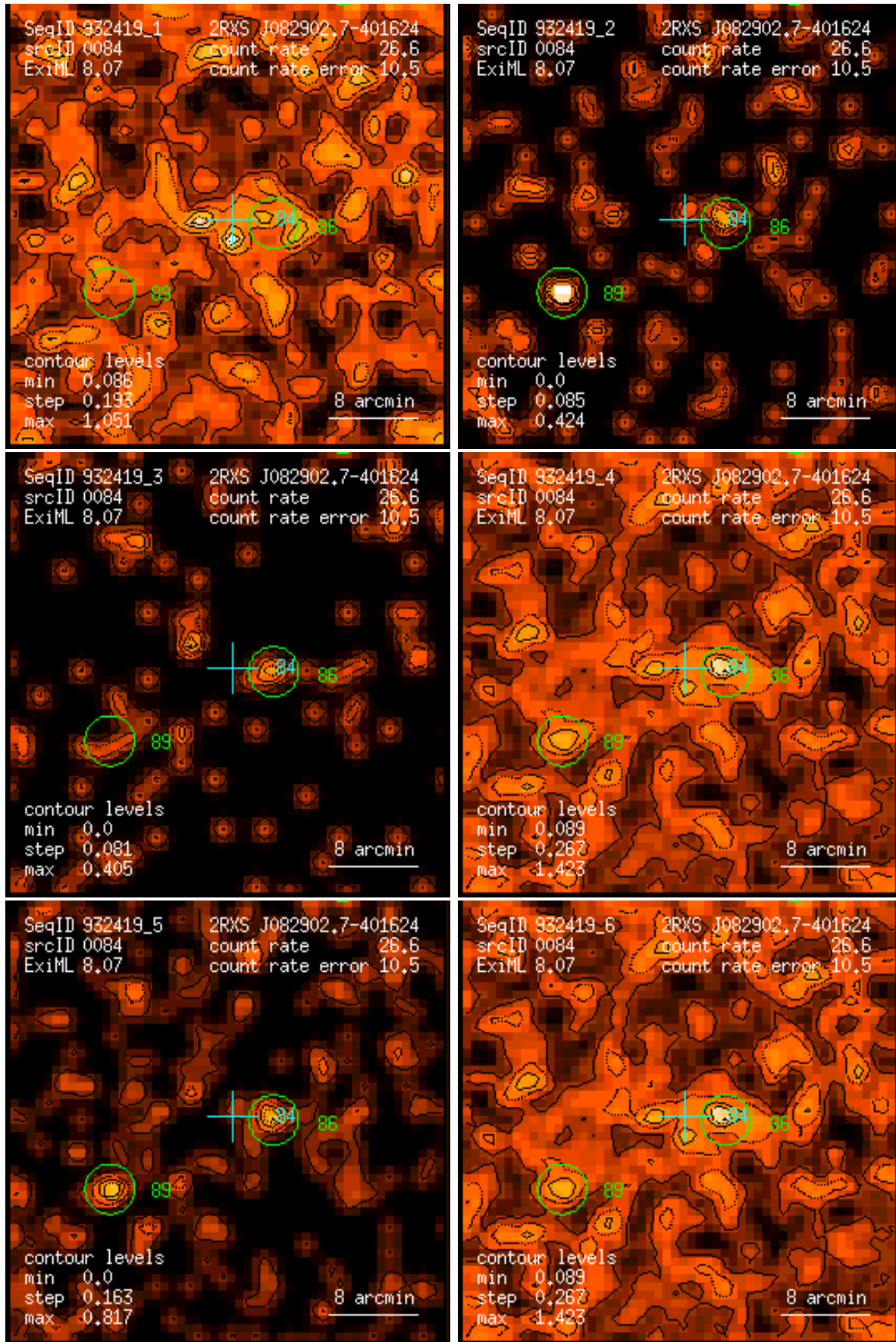
Figure 84: RASS 932419: detection 0084: band rate images, Gaussian filter: (1) PSPC channels 11 – 41, (2) 52 – 90, (3) 91 – 201, (4) 11 – 235, (5) 52 – 201, (6) 11 – 201. Broad band rates in counts/ks. Band rate contour levels in counts/ks/arcmin 2 .
