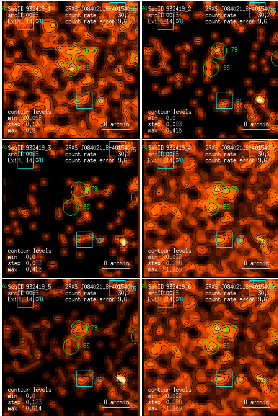
Figure 85: RASS 932419: detection 0085: band rate images, Gaussian filter: (1) PSPC channels 11 – 41, (2) 52 – 90, (3) 91 – 201, (4) 11 – 235, (5) 52 – 201, (6) 11 – 201. Broad band rates in counts/ks. Band rate contour levels in counts/ks/arcmin 2 .
