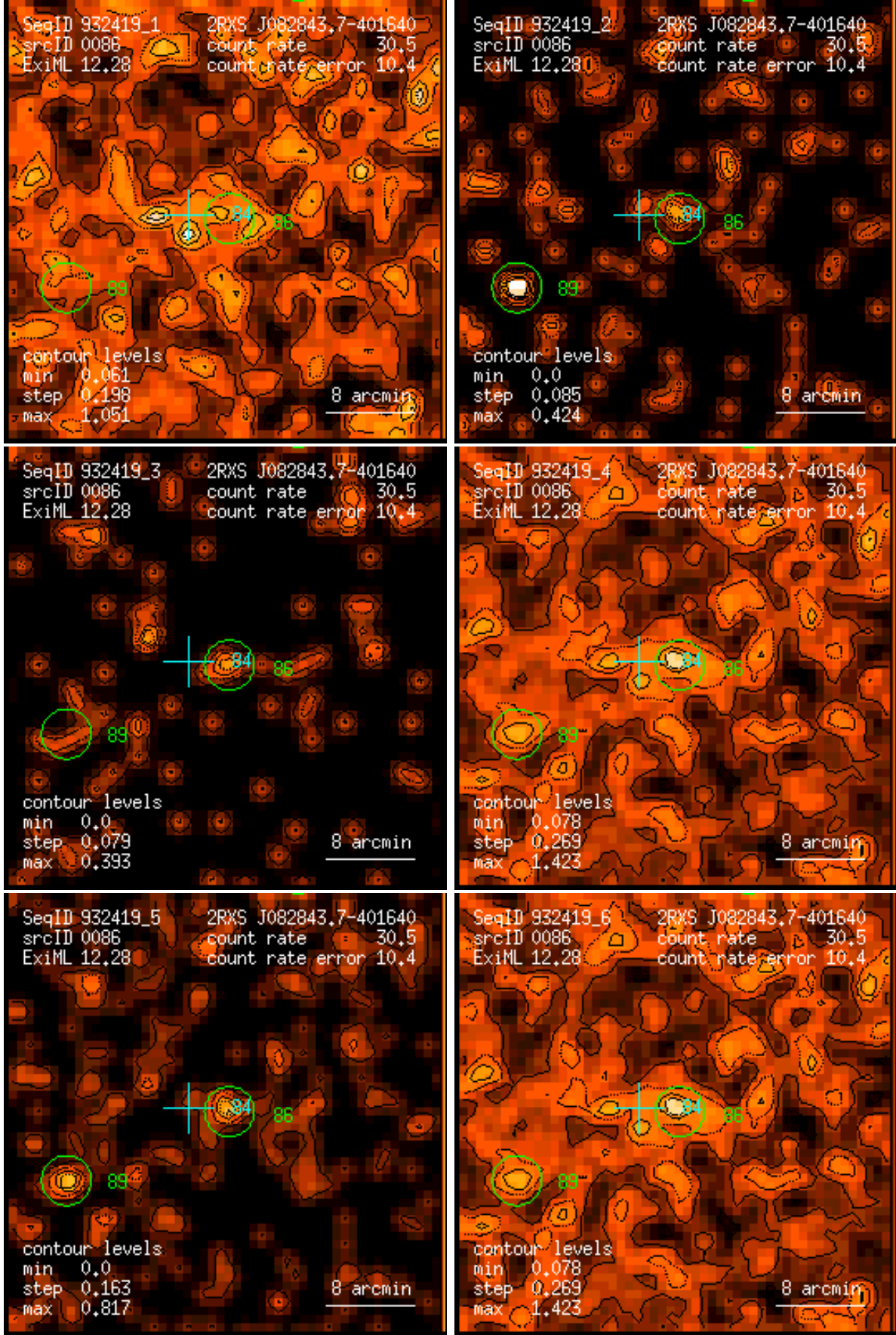
Figure 86: RASS 932419: detection 0086: band rate images, Gaussian filter: (1) PSPC channels 11 – 41, (2) 52 – 90, (3) 91 – 201, (4) 11 – 235, (5) 52 – 201, (6) 11 – 201. Broad band rates in counts/ks. Band rate contour levels in counts/ks/arcmin 2 .
