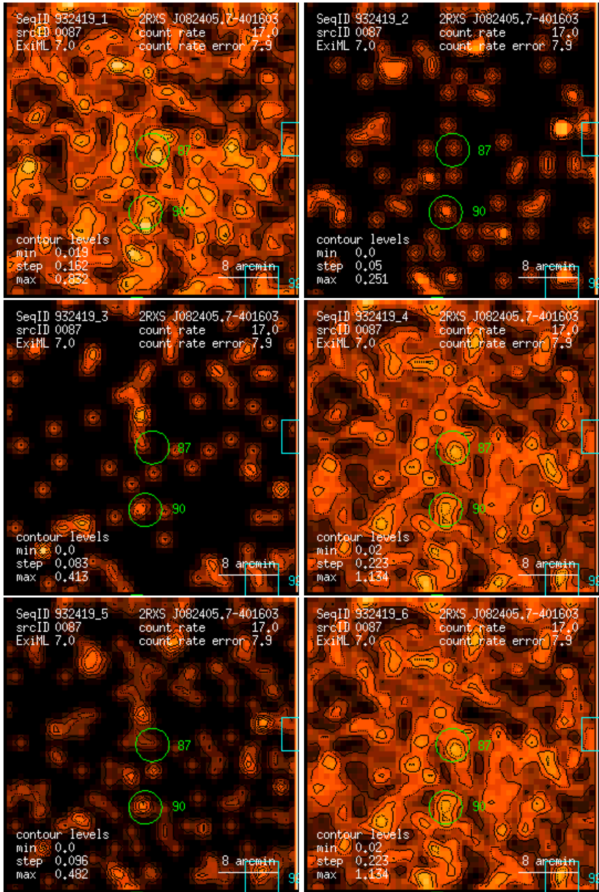
Figure 87: RASS 932419: detection 0087: band rate images, Gaussian filter: (1) PSPC channels 11 – 41, (2) 52 – 90, (3) 91 – 201, (4) 11 – 235, (5) 52 – 201, (6) 11 – 201. Broad band rates in counts/ks. Band rate contour levels in counts/ks/arcmin 2 .
