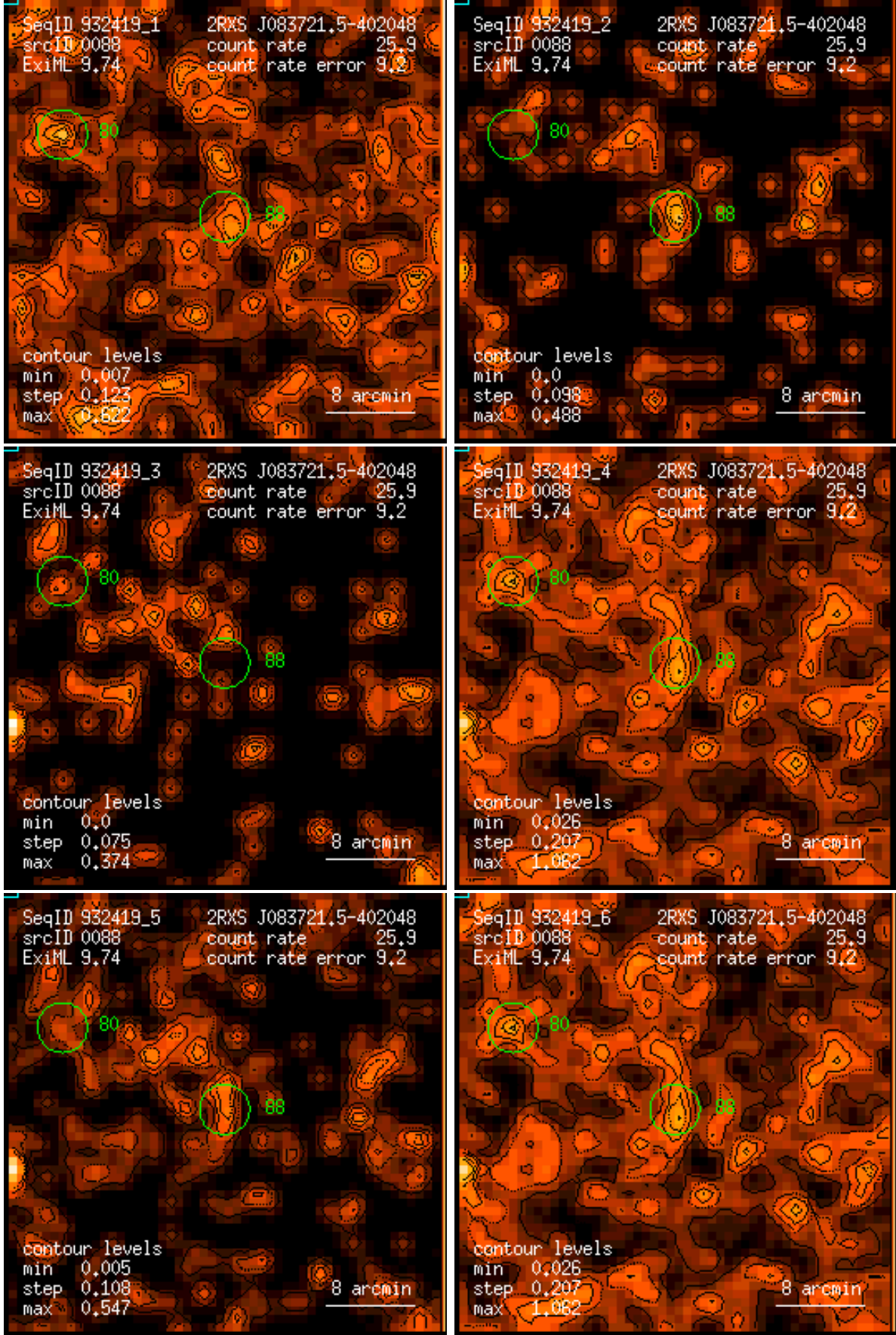
Figure 88: RASS 932419: detection 0088: band rate images, Gaussian filter: (1) PSPC channels 11 – 41, (2) 52 – 90, (3) 91 – 201, (4) 11 – 235, (5) 52 – 201, (6) 11 – 201. Broad band rates in counts/ks. Band rate contour levels in counts/ks/arcmin 2 .
