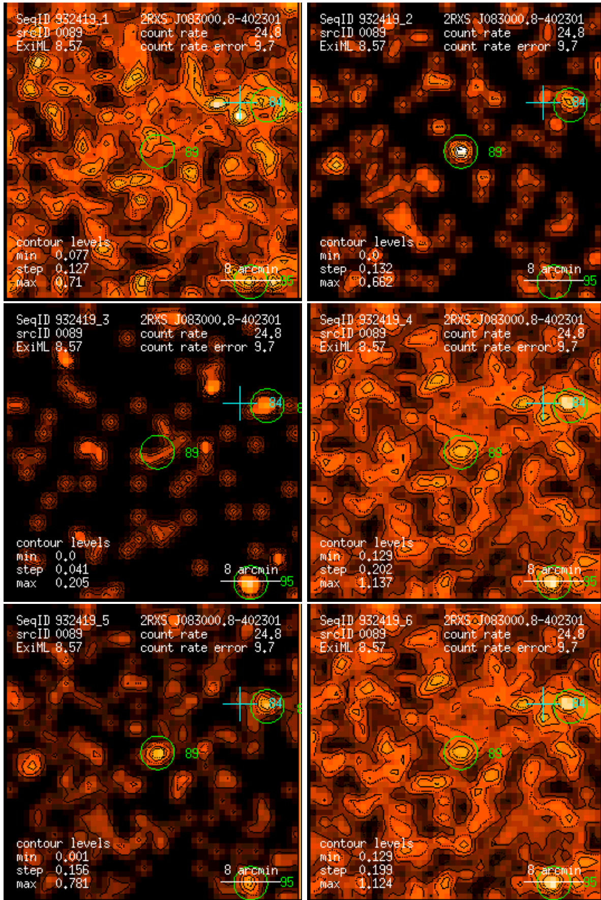
Figure 89: RASS 932419: detection 0089: band rate images, Gaussian filter: (1) PSPC channels 11 – 41, (2) 52 – 90, (3) 91 – 201, (4) 11 – 235, (5) 52 – 201, (6) 11 – 201. Broad band rates in counts/ks. Band rate contour levels in counts/ks/arcmin 2 .
