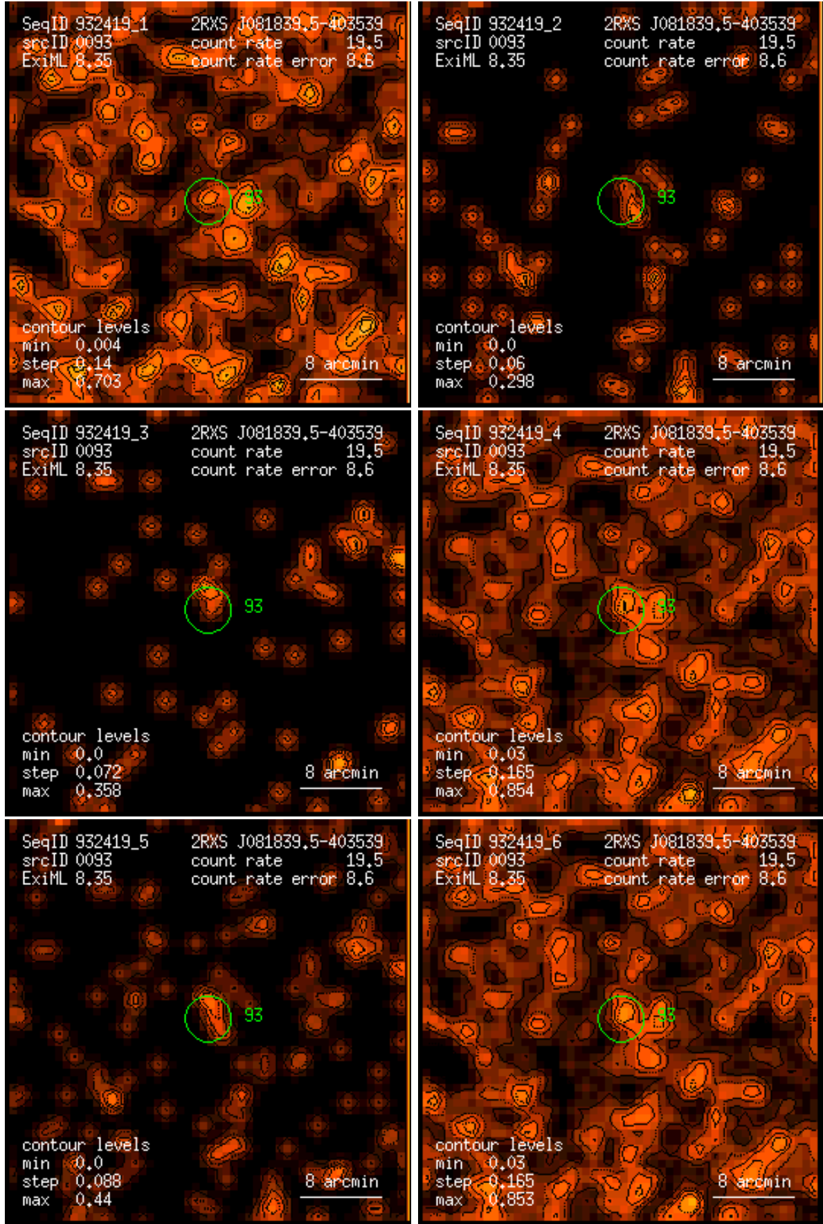
Figure 93: RASS 932419: detection 0093: band rate images, Gaussian filter: (1) PSPC channels 11 – 41, (2) 52 – 90, (3) 91 – 201, (4) 11 – 235, (5) 52 – 201, (6) 11 – 201. Broad band rates in counts/ks. Band rate contour levels in counts/ks/arcmin 2 .
