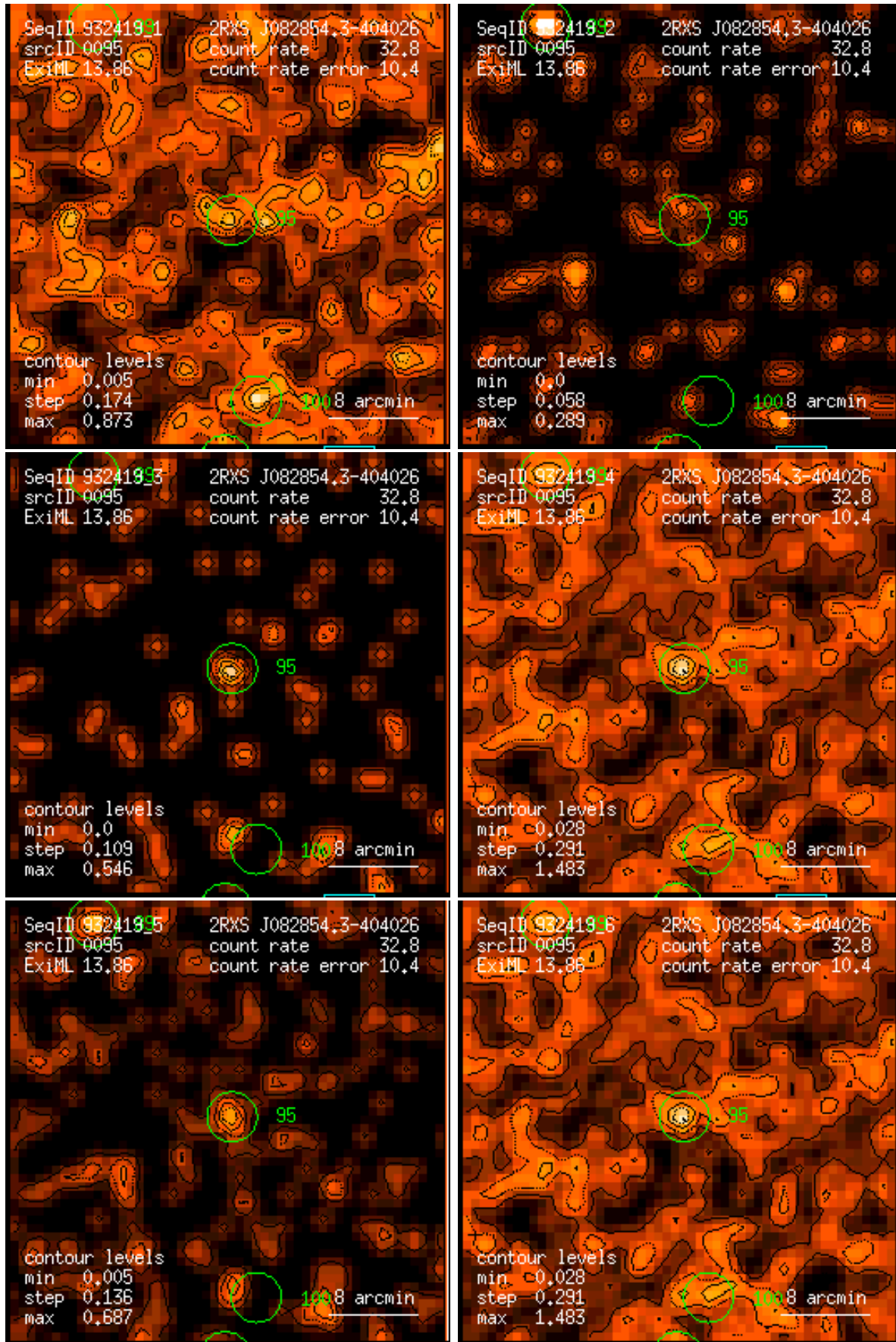
Figure 95: RASS 932419: detection 0095: band rate images, Gaussian filter: (1) PSPC channels 11 – 41, (2) 52 – 90, (3) 91 – 201, (4) 11 – 235, (5) 52 – 201, (6) 11 – 201. Broad band rates in counts/ks. Band rate contour levels in counts/ks/arcmin 2 .
