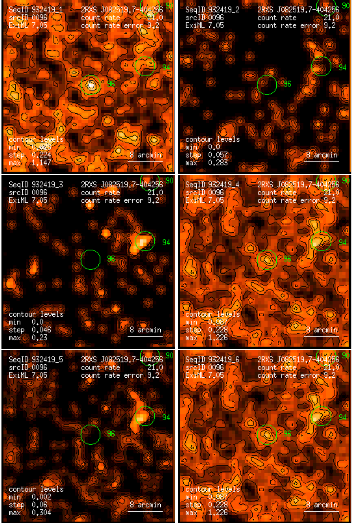
Figure 96: RASS 932419: detection 0096: band rate images, Gaussian filter: (1) PSPC channels 11 – 41, (2) 52 – 90, (3) 91 – 201, (4) 11 – 235, (5) 52 – 201, (6) 11 – 201. Broad band rates in counts/ks. Band rate contour levels in counts/ks/arcmin 2 .
