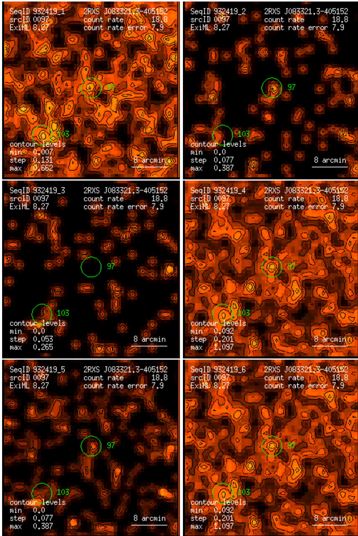
Figure 97: RASS 932419: detection 0097: band rate images, Gaussian filter: (1) PSPP channels 11 – 41, (2) 52 – 90, (3) 91 – 201, (4) 11 – 235, (5) 52 – 201, (6) 11 – 201. Broad band rates in counts/ks. Band rate contour levels in counts/ks/arcmin 2 .
