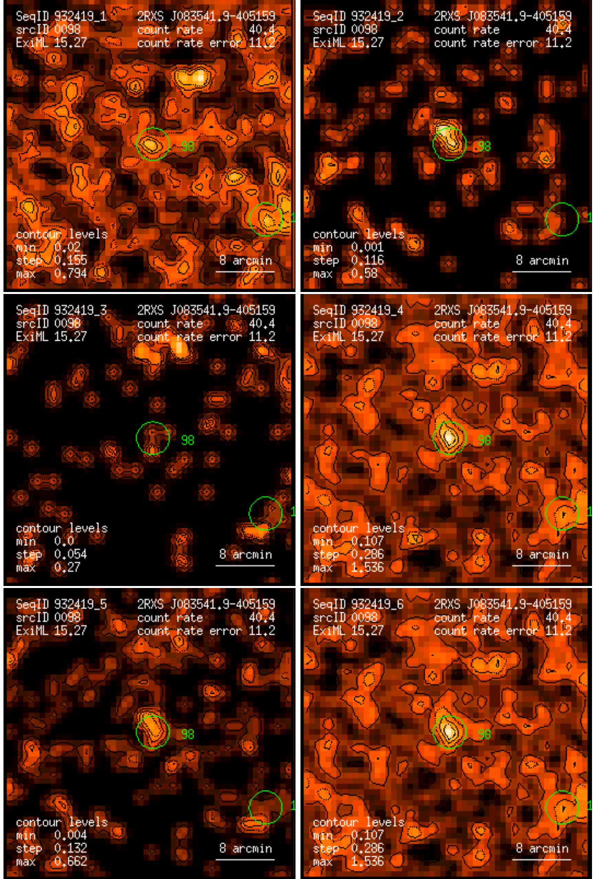
Figure 98: RASS 932419: detection 0098: band rate images, Gaussian filter: (1) PSPC channels 11 – 41, (2) 52 – 90, (3) 91 – 201, (4) 11 – 235, (5) 52 – 201, (6) 11 – 201. Broad band rates in counts/ks. Band rate contour levels in counts/ks/arcmin 2 .
