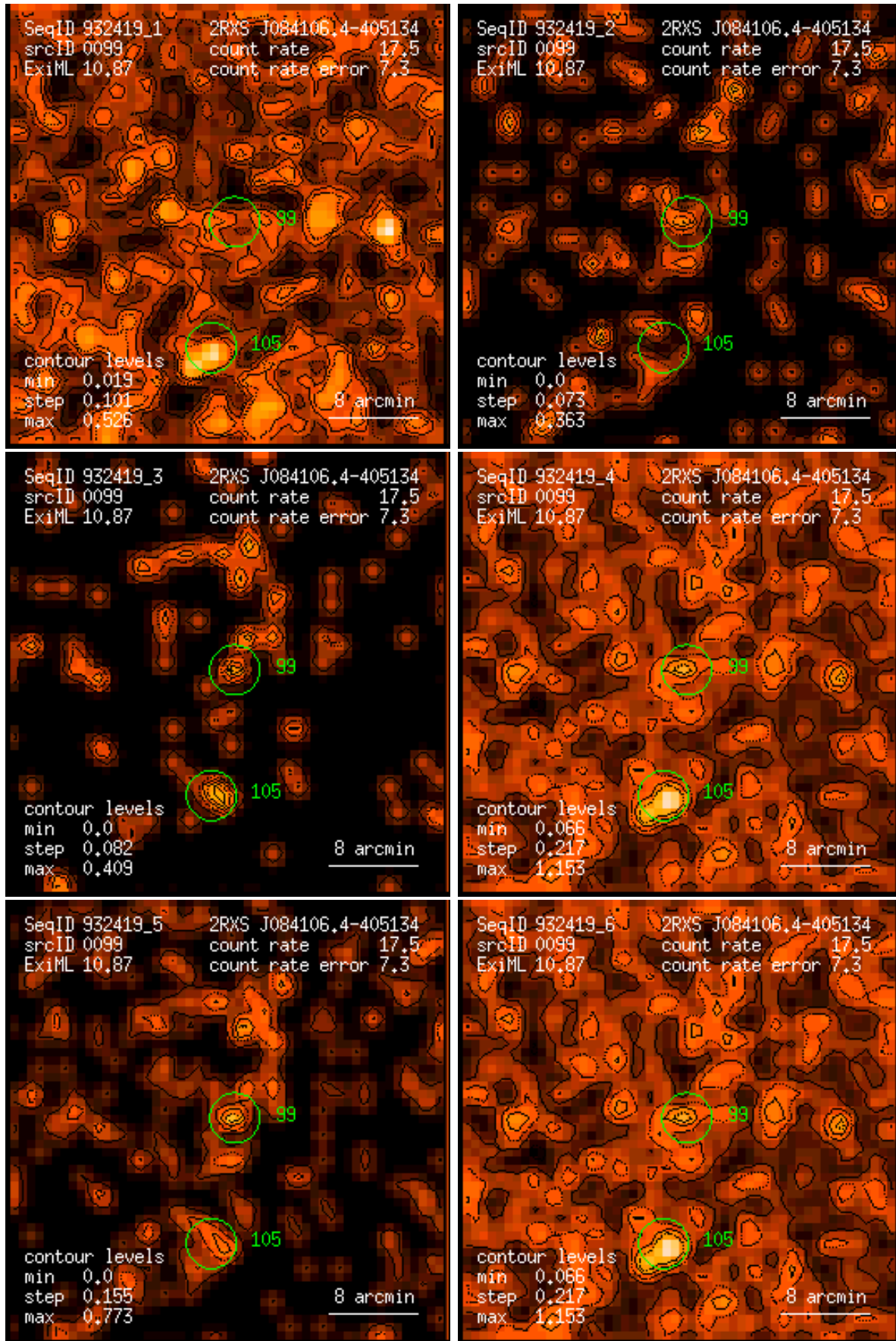
Figure 99: RASS 932419: detection 0099: band rate images, Gaussian filter: (1) PSPC channels 11 – 41, (2) 52 – 90, (3) 91 – 201, (4) 11 – 235, (5) 52 – 201, (6) 11 – 201. Broad band rates in counts/ks. Band rate contour levels in counts/ks/arcmin 2 .
