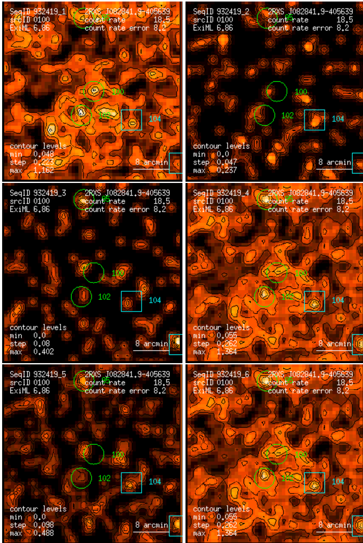
Figure 100: RASS 932419: detection 0100: band rate images, Gaussian filter: (1) PSPC channels 11 – 41, (2) 52 – 90, (3) 91 – 201, (4) 11 – 235, (5) 52 – 201, (6) 11 – 201. Broad band rates in counts/ks. Band rate contour levels in counts/ks/arcmin 2 .
