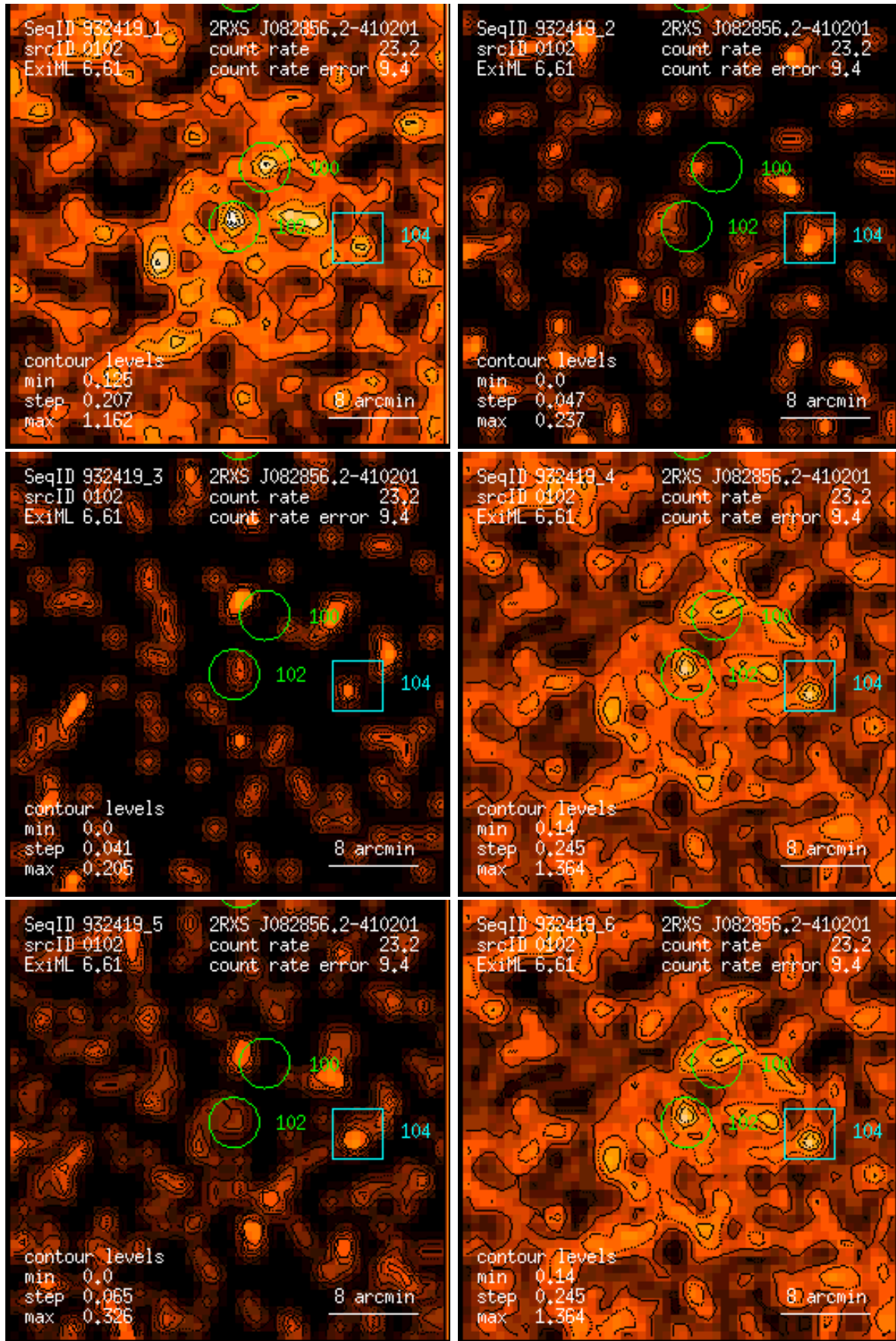
Figure 102: RASS 932419: detection 0102: band rate images, Gaussian filter: (1) PSPC channels 11 – 41, (2) 52 – 90, (3) 91 – 201, (4) 11 – 235, (5) 52 – 201, (6) 11 – 201. Broad band rates in counts/ks. Band rate contour levels in counts/ks/arcmin 2 .
