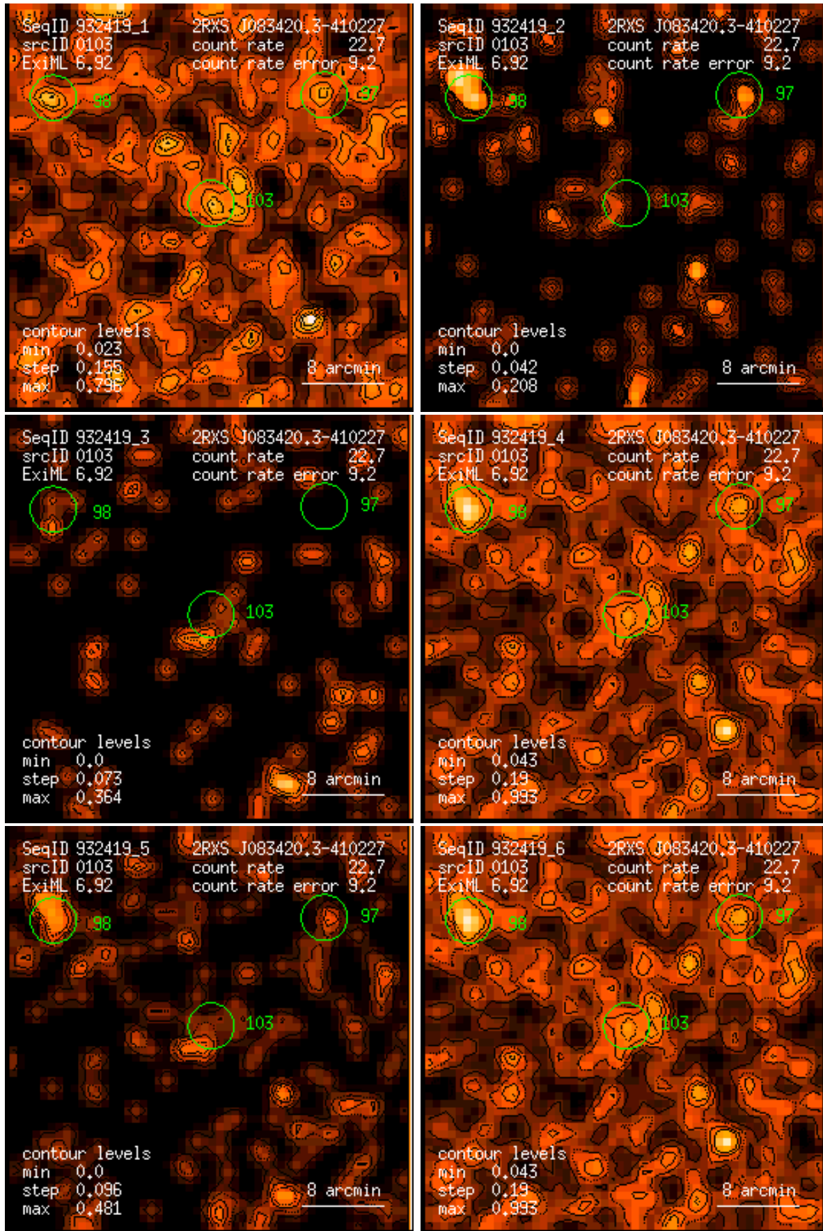
Figure 103: RASS 932419: detection 0103: band rate images, Gaussian filter: (1) PSPC channels 11 – 41, (2) 52 – 90, (3) 91 – 201, (4) 11 – 235, (5) 52 – 201, (6) 11 – 201. Broad band rates in counts/ks. Band rate contour levels in counts/ks/arcmin 2 .
