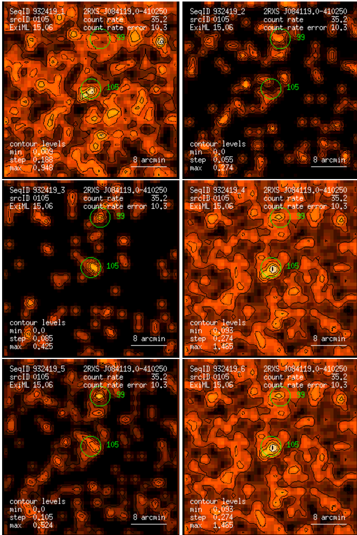
Figure 105: RASS 932419: detection 0105: band rate images, Gaussian filter: (1) PSPC channels 11 – 41, (2) 52 – 90, (3) 91 – 201, (4) 11 – 235, (5) 52 – 201, (6) 11 – 201. Broad band rates in counts/ks. Band rate contour levels in counts/ks/arcmin 2 .
