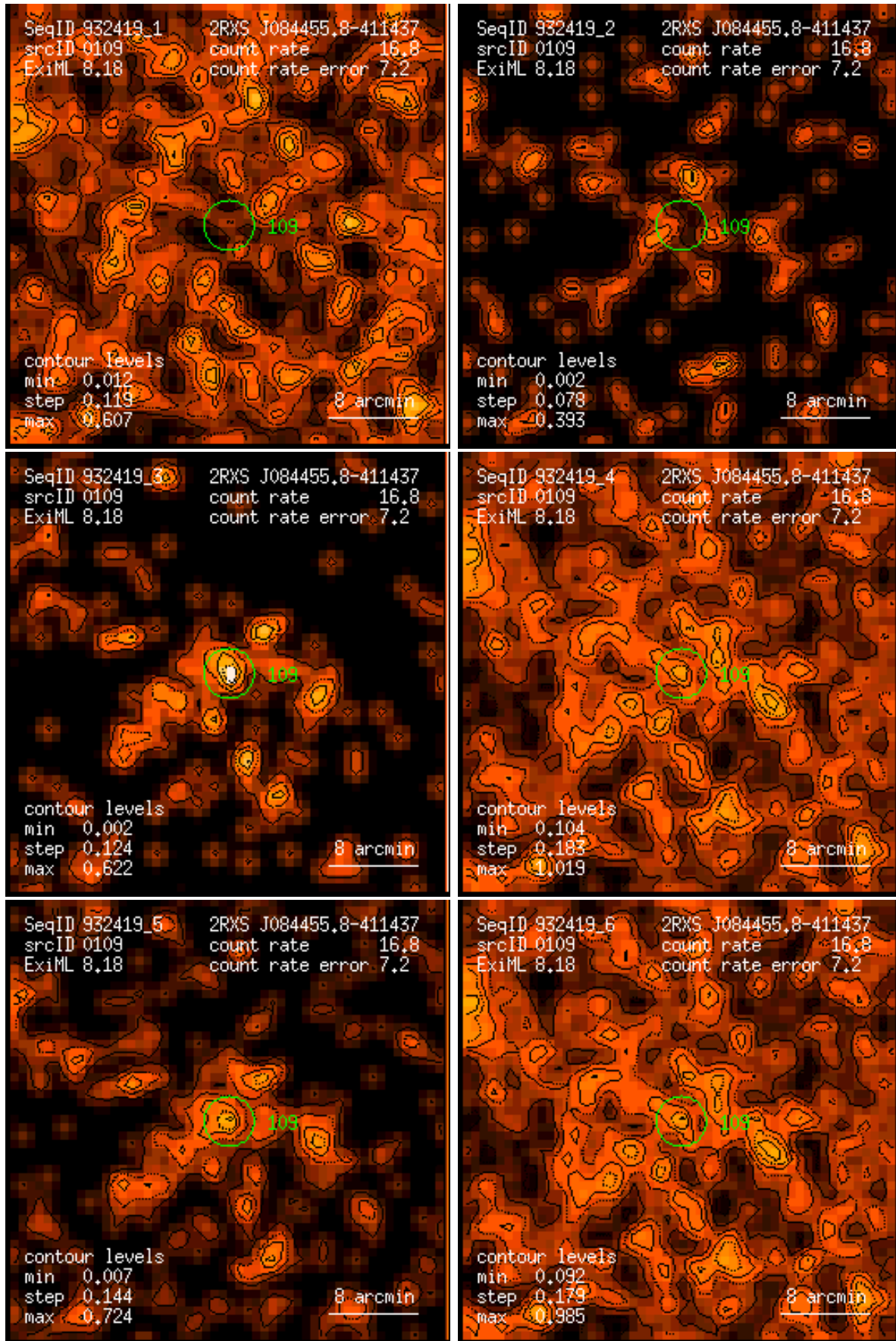
Figure 109: RASS 932419: detection 0109: band rate images, Gaussian filter: (1) PSPC channels 11 – 41, (2) 52 – 90, (3) 91 – 201, (4) 11 – 235, (5) 52 – 201, (6) 11 – 201. Broad band rates in counts/ks. Band rate contour levels in counts/ks/arcmin 2 .
