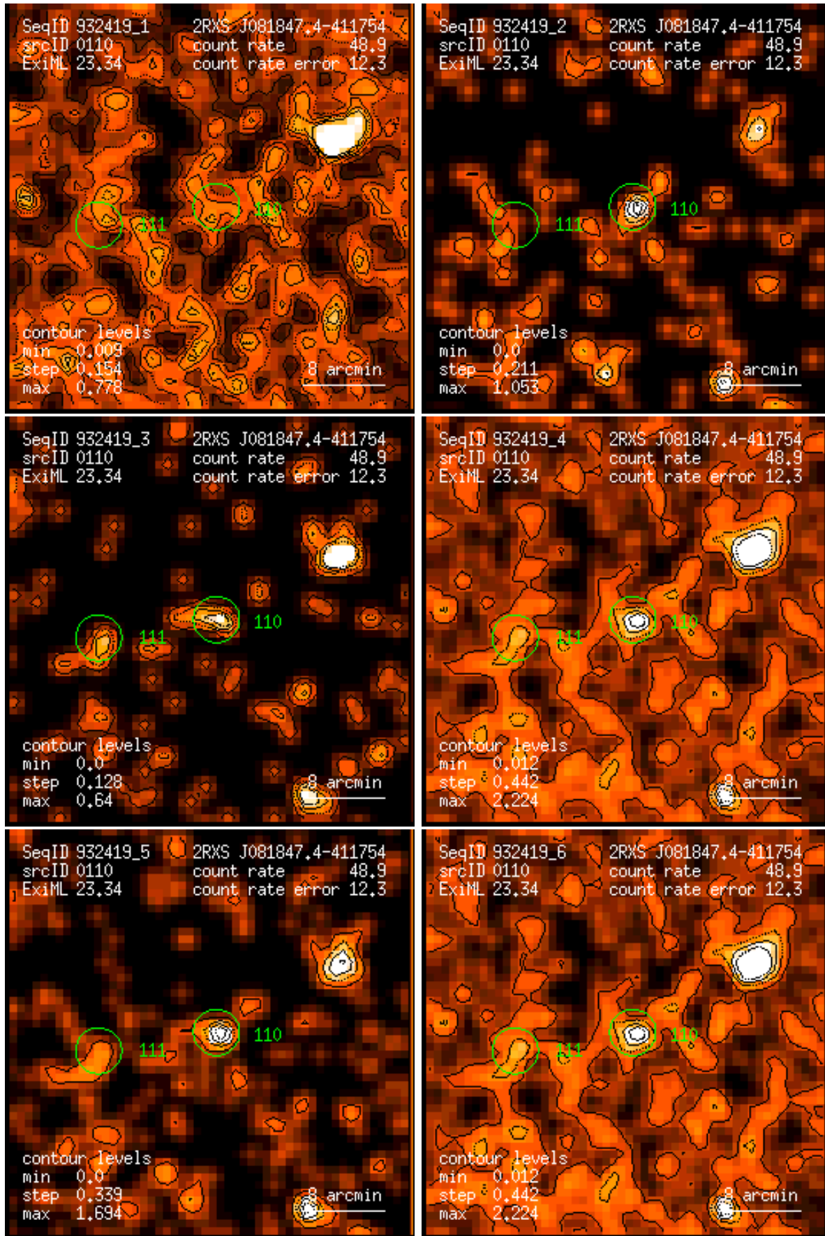
Figure 110: RASS 932419: detection 0110: band rate images, Gaussian filter: (1) PSPC channels 11 – 41, (2) 52 – 90, (3) 91 – 201, (4) 11 – 235, (5) 52 – 201, (6) 11 – 201. Broad band rates in counts/ks. Band rate contour levels in counts/ks/arcmin 2 .
