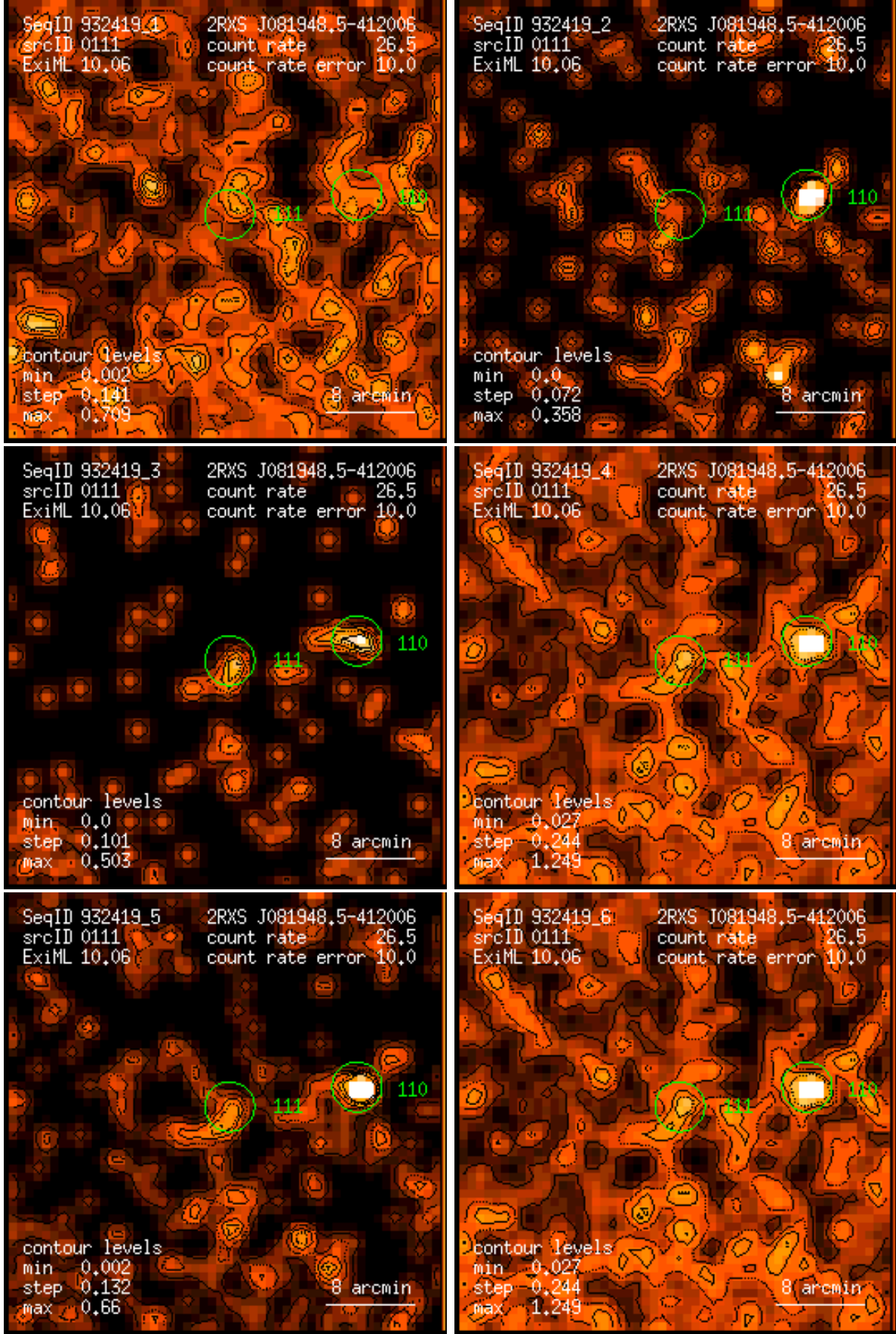
Figure 111: RASS 932419: detection 0111: band rate images, Gaussian filter: (1) PSPC channels 11 – 41, (2) 52 – 90, (3) 91 – 201, (4) 11 – 235, (5) 52 – 201, (6) 11 – 201. Broad band rates in counts/ks. Band rate contour levels in counts/ks/arcmin 2 .
