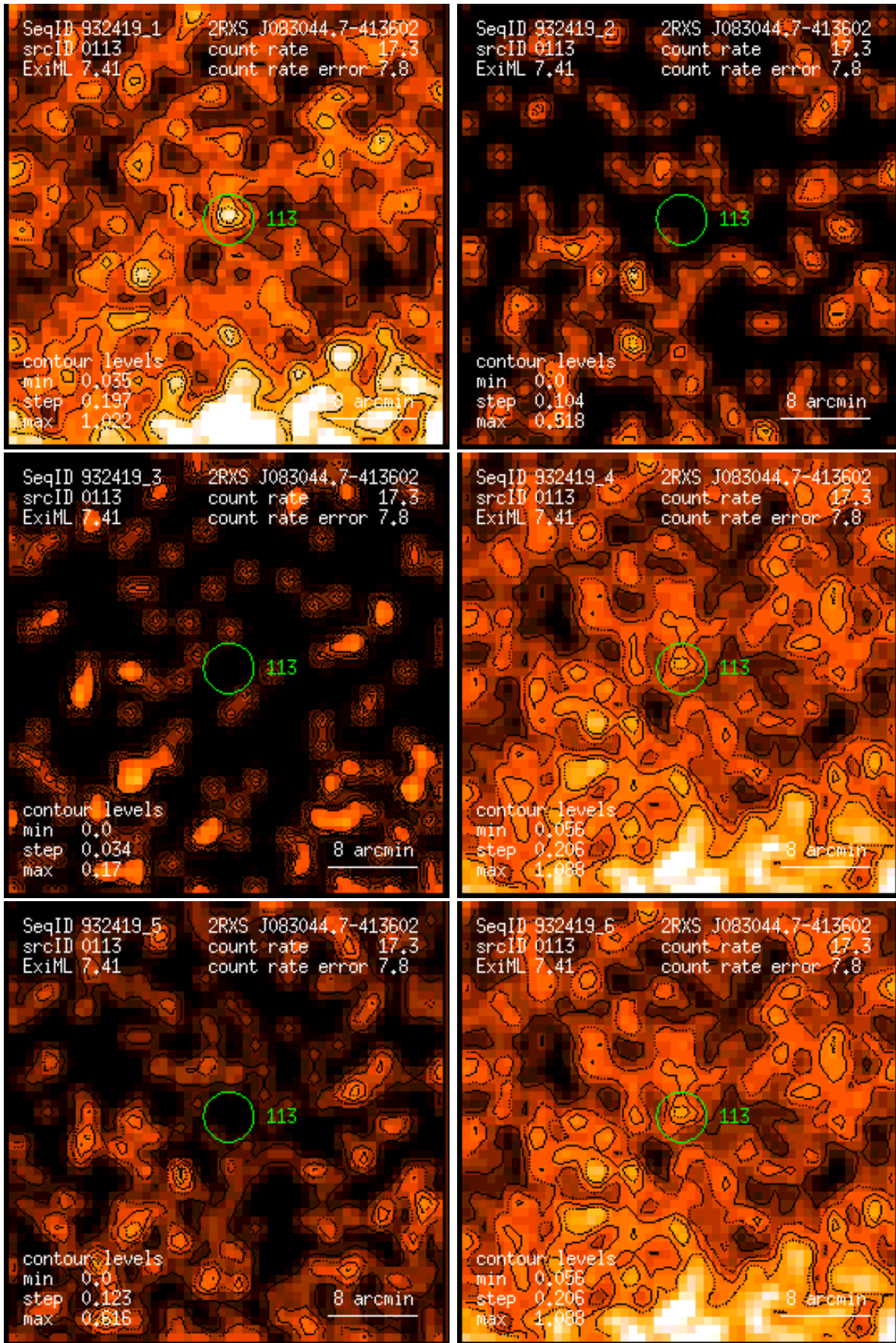
Figure 113: RASS 932419: detection 0113: band rate images, Gaussian filter: (1) PSPC channels 11 – 41, (2) 52 – 90, (3) 91 – 201, (4) 11 – 235, (5) 52 – 201, (6) 11 – 201. Broad band rates in counts/ks. Band rate contour levels in counts/ks/arcmin 2 .
