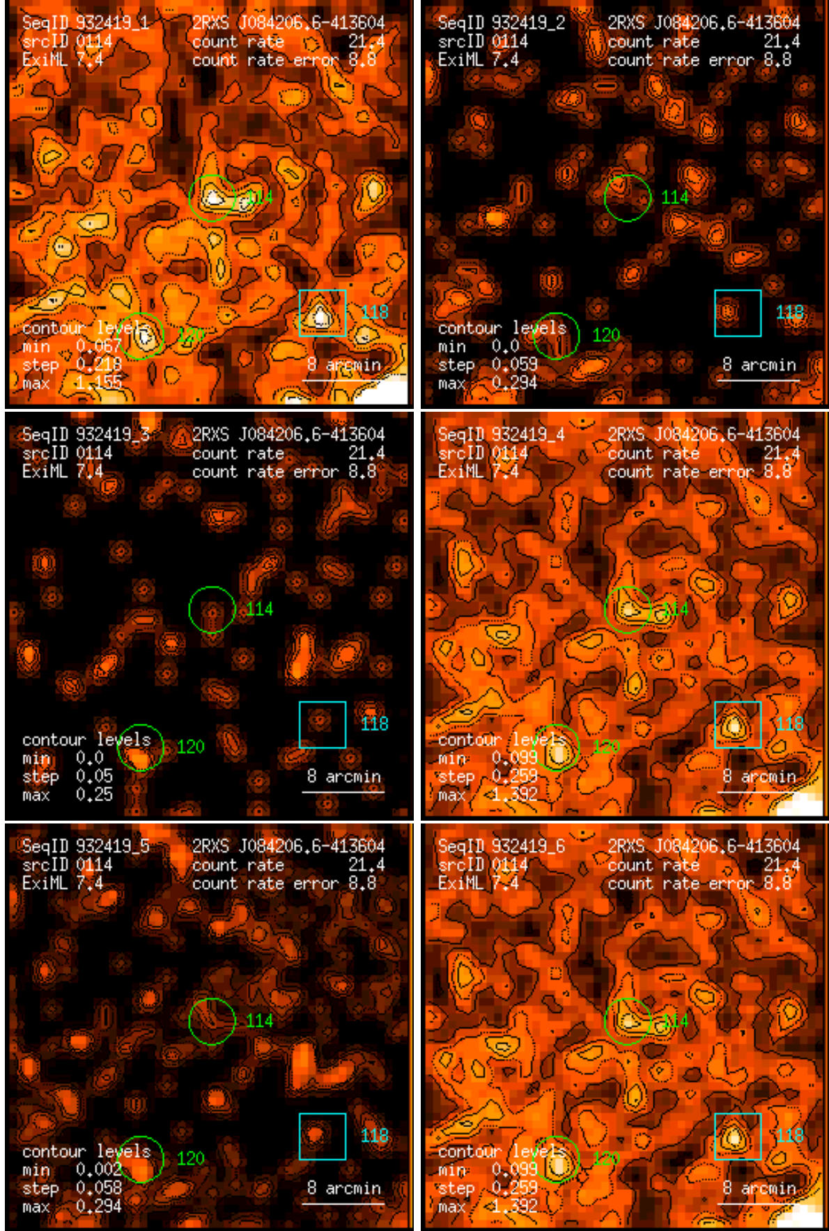
Figure 114: RASS 932419: detection 0114: band rate images, Gaussian filter: (1) PSPC channels 11 – 41, (2) 52 – 90, (3) 91 – 201, (4) 11 – 235, (5) 52 – 201, (6) 11 – 201. Broad band rates in counts/ks. Band rate contour levels in counts/ks/arcmin 2 .
