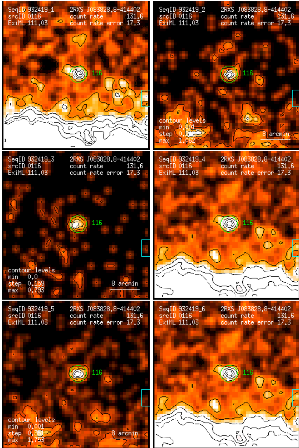
Figure 116: RASS 932419: detection 0116: band rate images, Gaussian filter: (1) PSPC channels 11 – 41, (2) 52 – 90, (3) 91 – 201, (4) 11 – 235, (5) 52 – 201, (6) 11 – 201. Broad band rates in counts/ks. Band rate contour levels in counts/ks/arcmin 2 .
