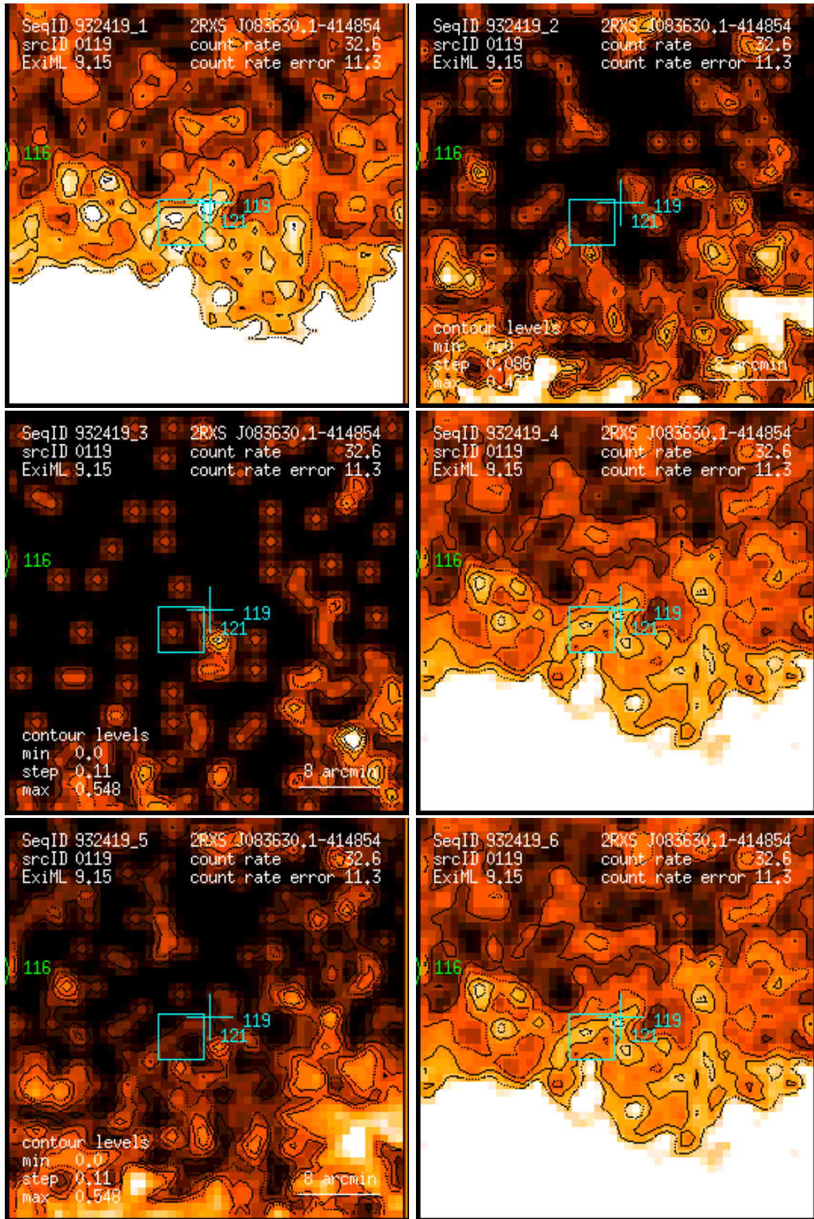
Figure 119: RASS 932419: detection 0119: band rate images, Gaussian filter: (1) PSPC channels 11 – 41, (2) 52 – 90, (3) 91 – 201, (4) 11 – 235, (5) 52 – 201, (6) 11 – 201. Broad band rates in counts/ks. Band rate contour levels in counts/ks/arcmin 2 .
