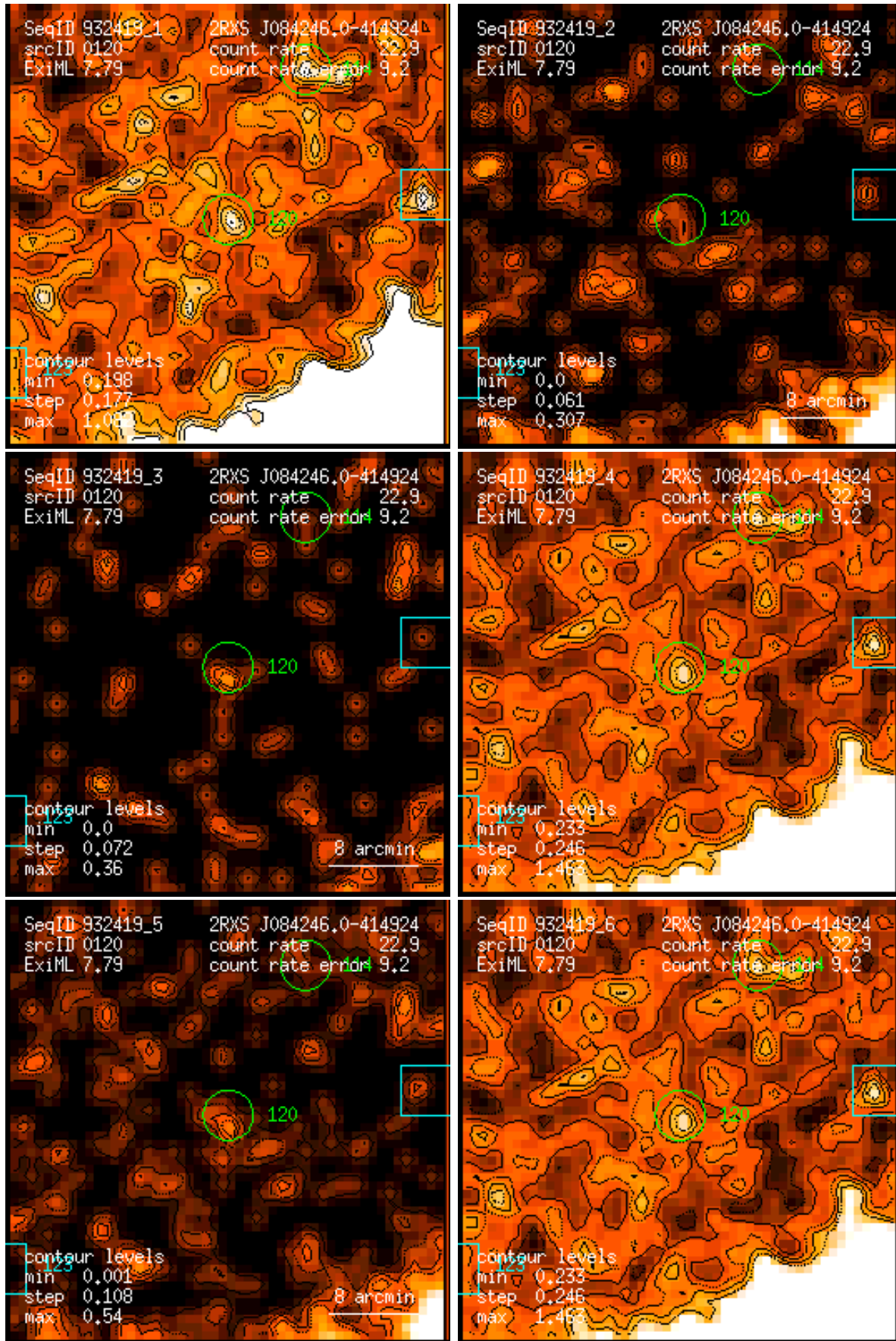
Figure 120: RASS 932419: detection 0120: band rate images, Gaussian filter: (1) PSPC channels 11 – 41, (2) 52 – 90, (3) 91 – 201, (4) 11 – 235, (5) 52 – 201, (6) 11 – 201. Broad band rates in counts/ks. Band rate contour levels in counts/ks/arcmin 2 .
