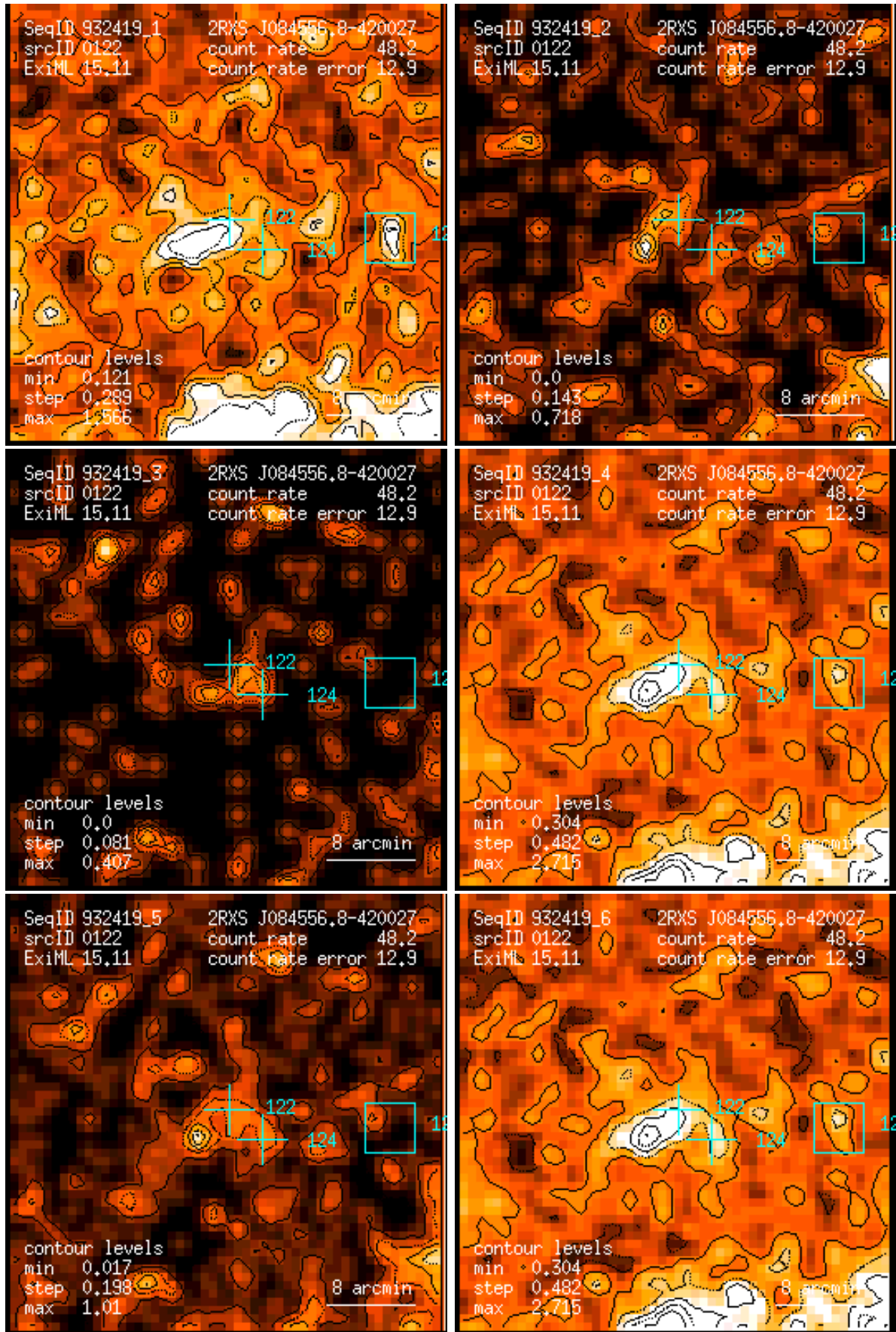
Figure 122: RASS 932419: detection 0122: band rate images, Gaussian filter: (1) PSPC channels 11 – 41, (2) 52 – 90, (3) 91 – 201, (4) 11 – 235, (5) 52 – 201, (6) 11 – 201. Broad band rates in counts/ks. Band rate contour levels in counts/ks/arcmin 2 .
