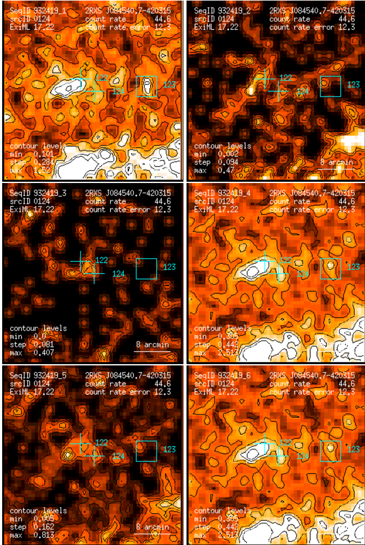
Figure 124: RASS 932419: detection 0124: band rate images, Gaussian filter: (1) PSPC channels 11 – 41, (2) 52 – 90, (3) 91 – 201, (4) 11 – 235, (5) 52 – 201, (6) 11 – 201. Broad band rates in counts/ks. Band rate contour levels in counts/ks/arcmin 2 .
