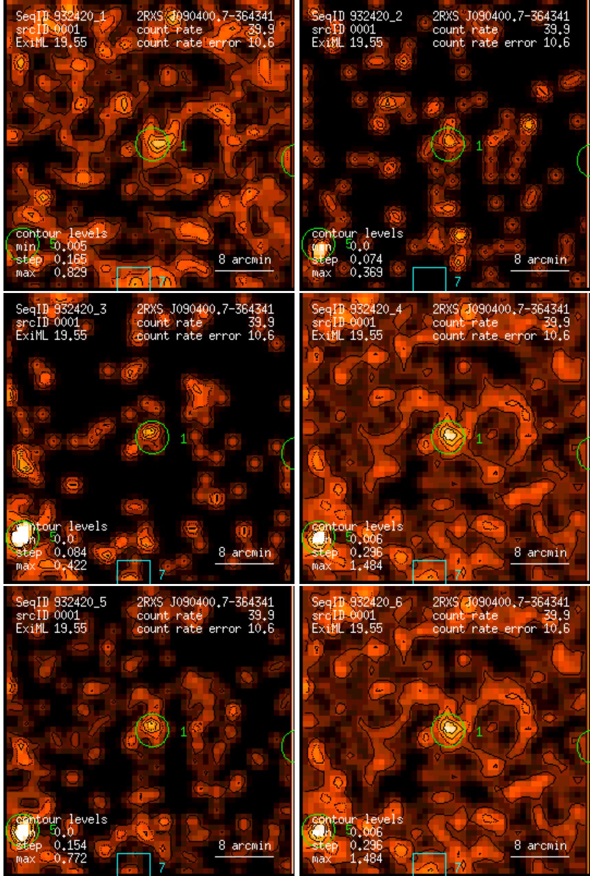
Figure 1: RASS 932420: detection 0001: band rate images, Gaussian filter: (1) PSPC channels 11 – 41, (2) 52 – 90, (3) 91 – 201, (4) 11 – 235, (5) 52 – 201, (6) 11 – 201. Broad band rates in counts/ks. Band rate contour levels in counts/ks/arcmin 2 .
