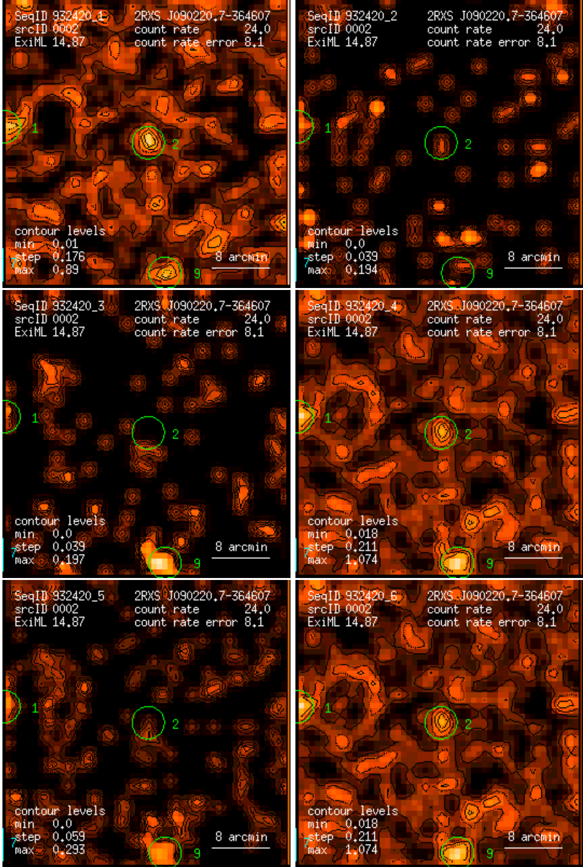
Figure 2: RASS 932420: detection 0002: band rate images, Gaussian filter: (1) PSPC channels 11 – 41, (2) 52 – 90, (3) 91 – 201, (4) 11 – 235, (5) 52 – 201, (6) 11 – 201. Broad band rates in counts/ks. Band rate contour levels in counts/ks/arcmin 2 .
