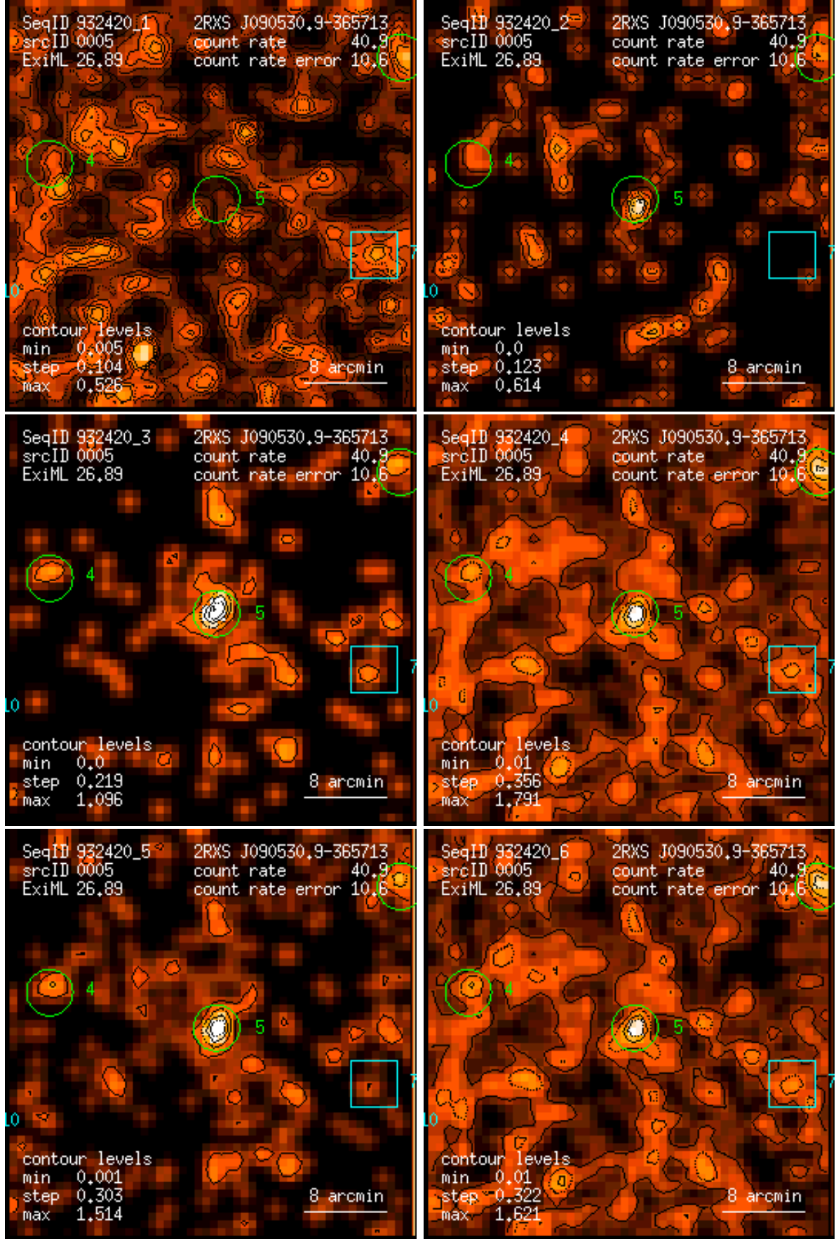
Figure 5: RASS 932420: detection 0005: band rate images, Gaussian filter: (1) PSPC channels 11 – 41, (2) 52 – 90, (3) 91 – 201, (4) 11 – 235, (5) 52 – 201, (6) 11 – 201. Broad band rates in counts/ks. Band rate contour levels in counts/ks/arcmin 2 .
