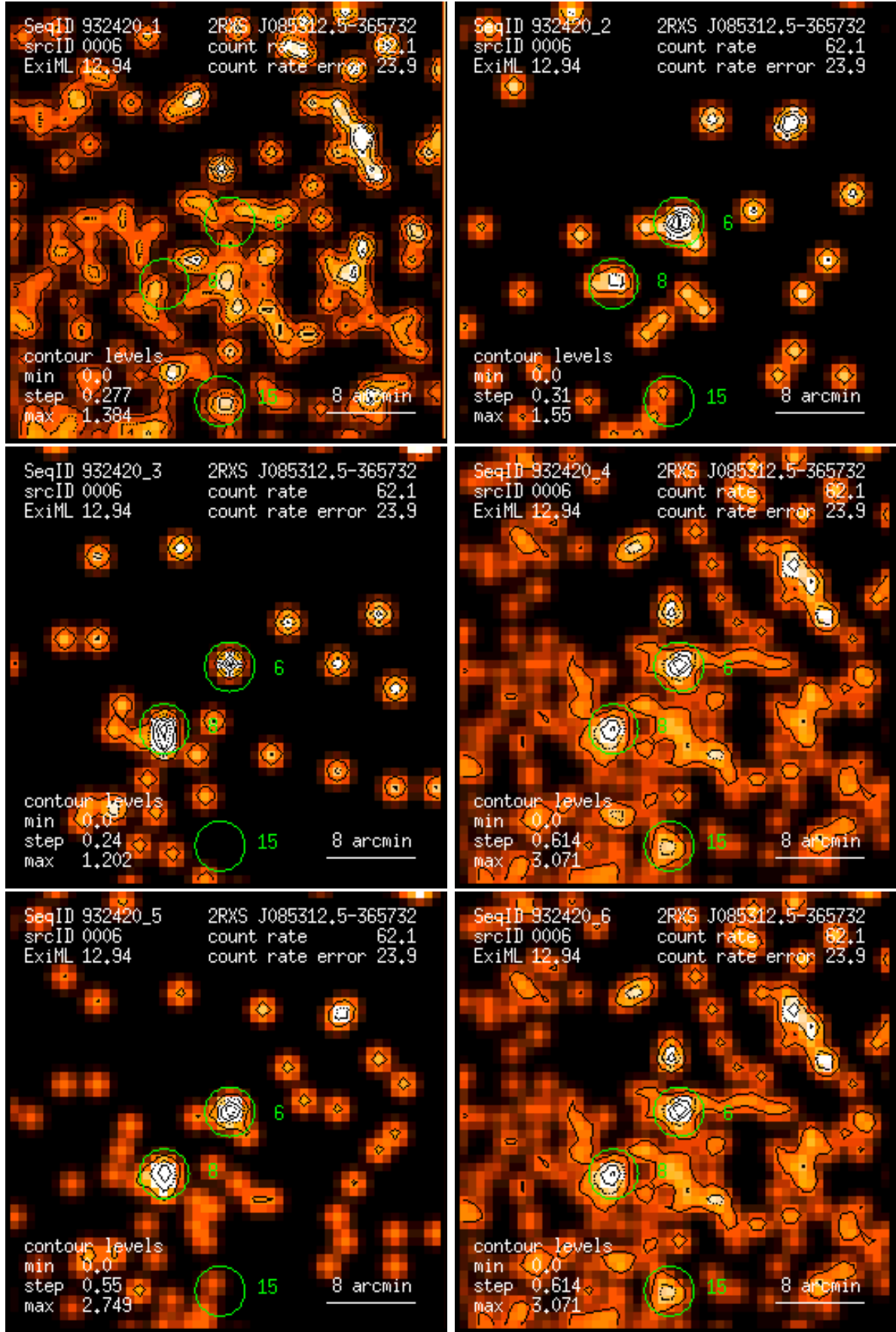
Figure 6: RASS 932420: detection 0006: band rate images, Gaussian filter: (1) PSPC channels 11 – 41, (2) 52 – 90, (3) 91 – 201, (4) 11 – 235, (5) 52 – 201, (6) 11 – 201. Broad band rates in counts/ks. Band rate contour levels in counts/ks/arcmin 2 .
