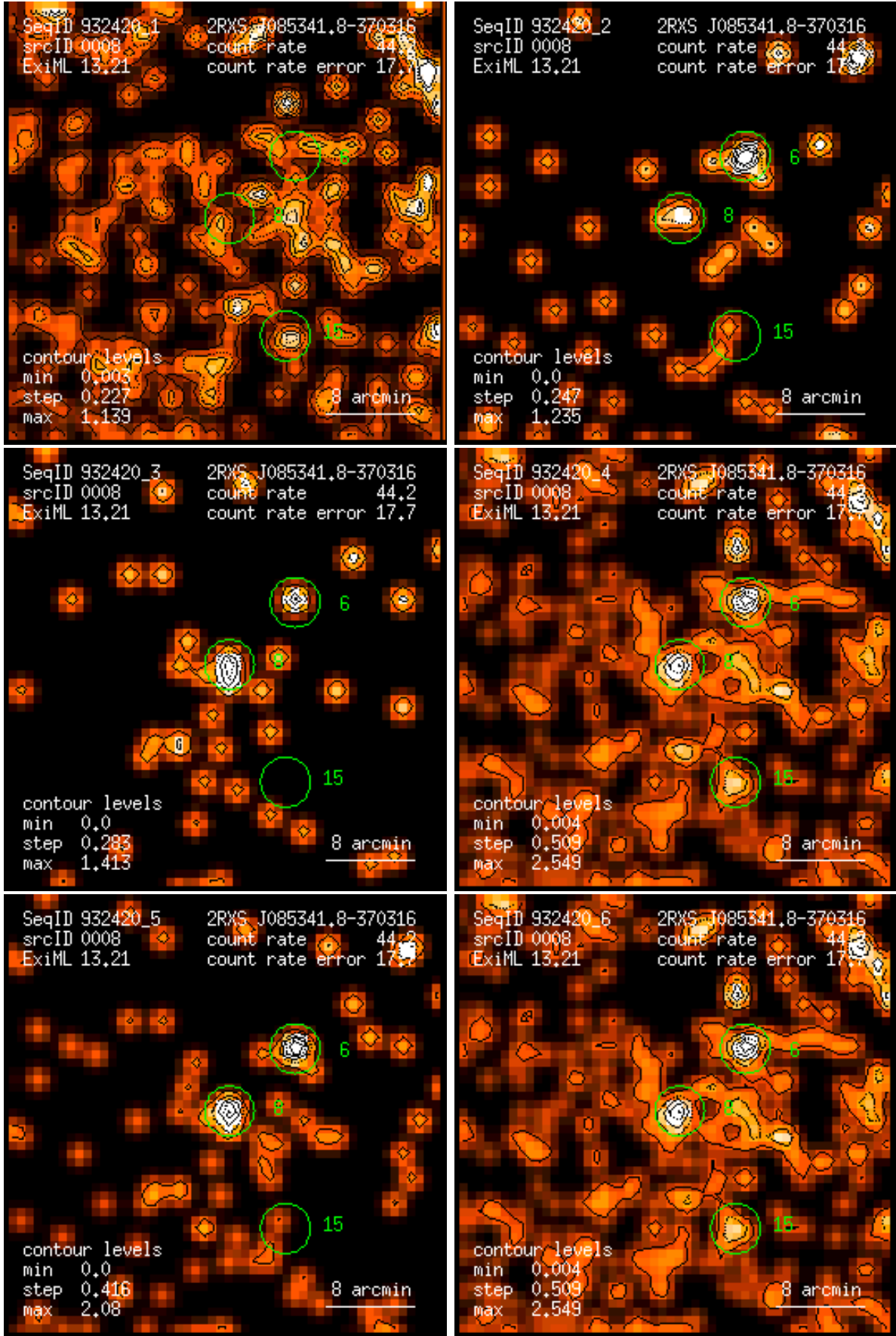
Figure 8: RASS 932420: detection 0008: band rate images, Gaussian filter: (1) PSPC channels 11 – 41, (2) 52 – 90, (3) 91 – 201, (4) 11 – 235, (5) 52 – 201, (6) 11 – 201. Broad band rates in counts/ks. Band rate contour levels in counts/ks/arcmin 2 .
