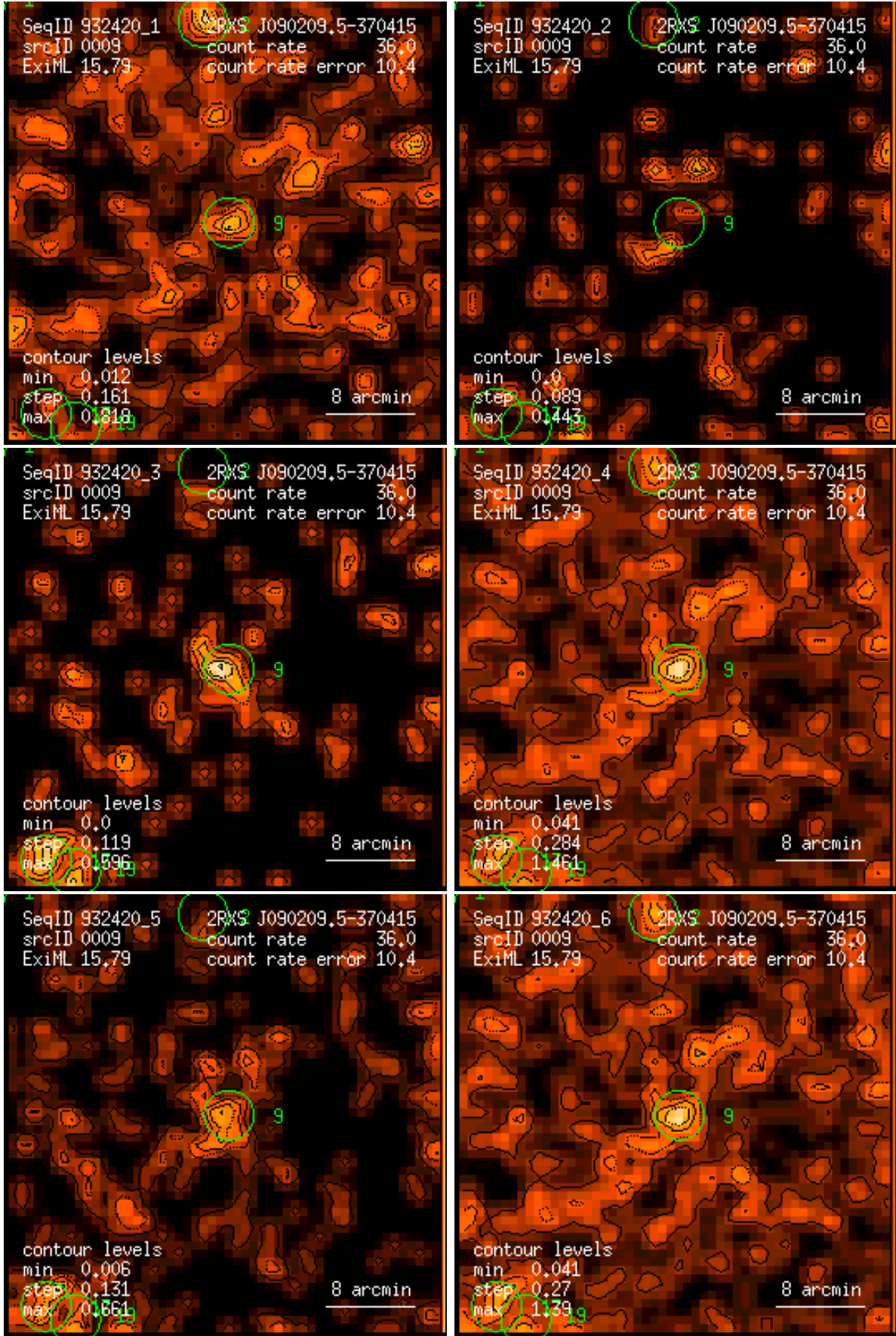
Figure 9: RASS 932420: detection 0009: band rate images, Gaussian filter: (1) PSPC channels 11 – 41, (2) 52 – 90, (3) 91 – 201, (4) 11 – 235, (5) 52 – 201, (6) 11 – 201. Broad band rates in counts/ks. Band rate contour levels in counts/ks/arcmin 2 .
