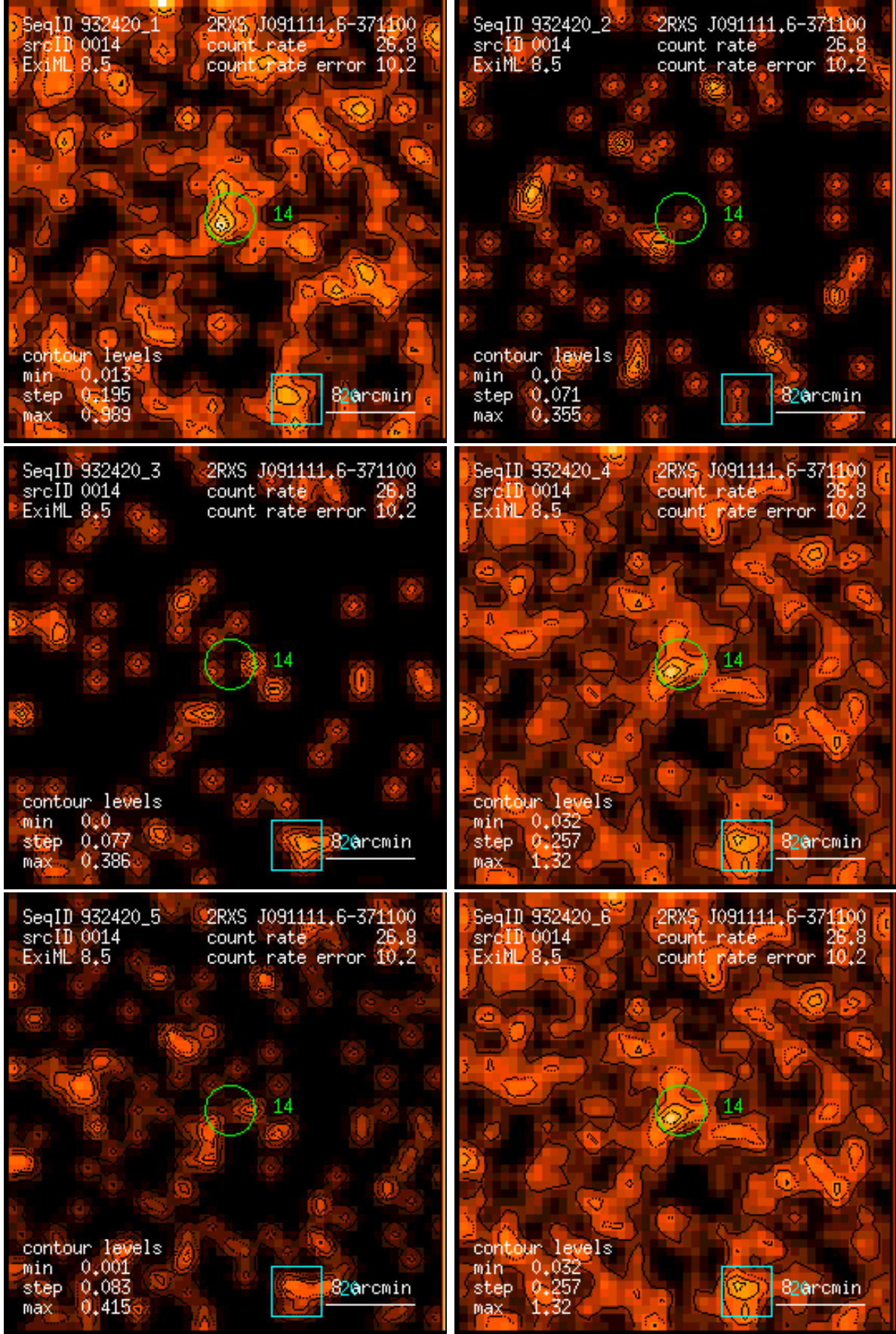
Figure 14: RASS 932420: detection 0014: band rate images, Gaussian filter: (1) PSPC channels 11 – 41, (2) 52 – 90, (3) 91 – 201, (4) 11 – 235, (5) 52 – 201, (6) 11 – 201. Broad band rates in counts/ks. Band rate contour levels in counts/ks/arcmin 2 .
