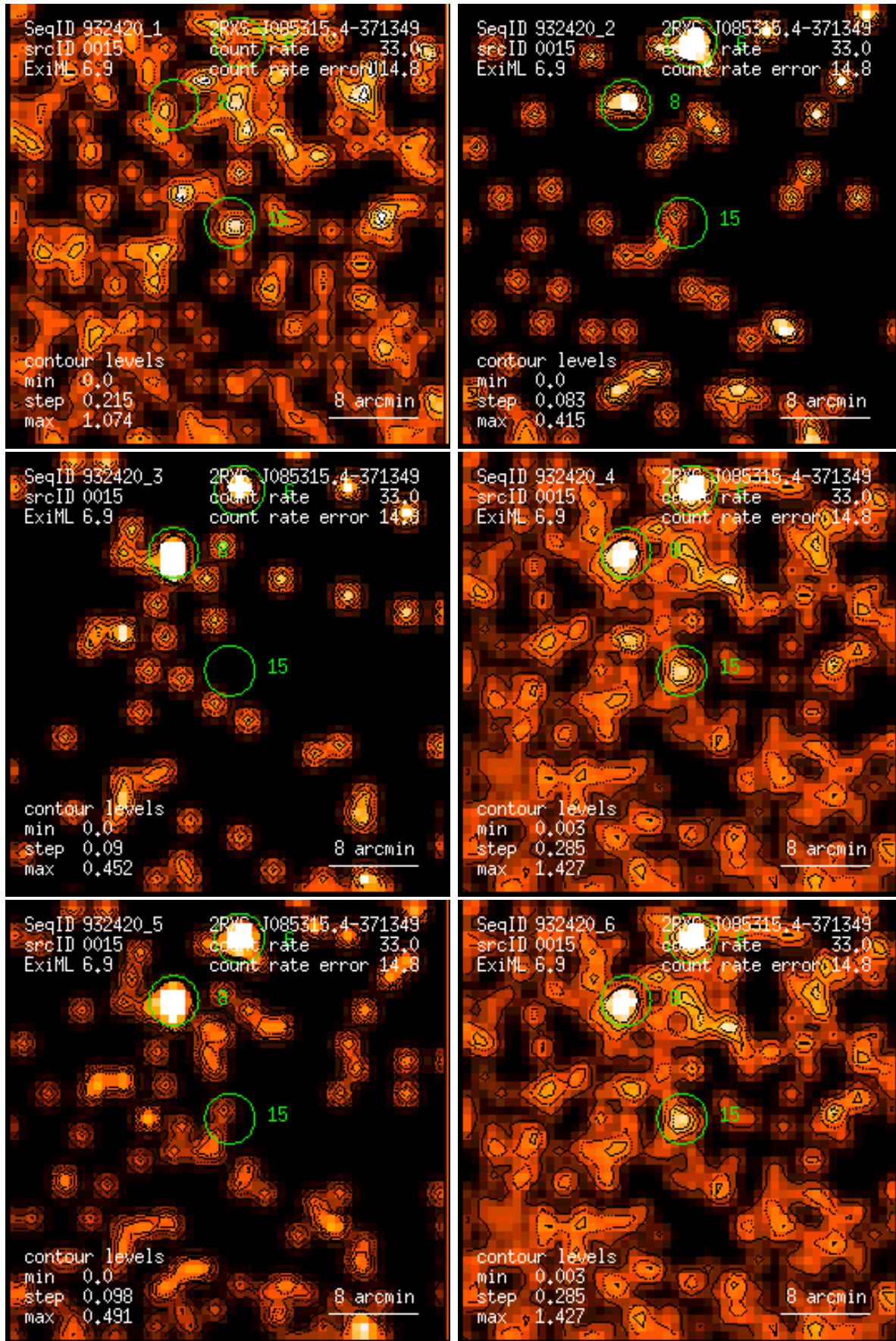
Figure 15: RASS 932420: detection 0015: band rate images, Gaussian filter: (1) PSPC channels 11 – 41, (2) 52 – 90, (3) 91 – 201, (4) 11 – 235, (5) 52 – 201, (6) 11 – 201. Broad band rates in counts/ks. Band rate contour levels in counts/ks/arcmin 2 .
