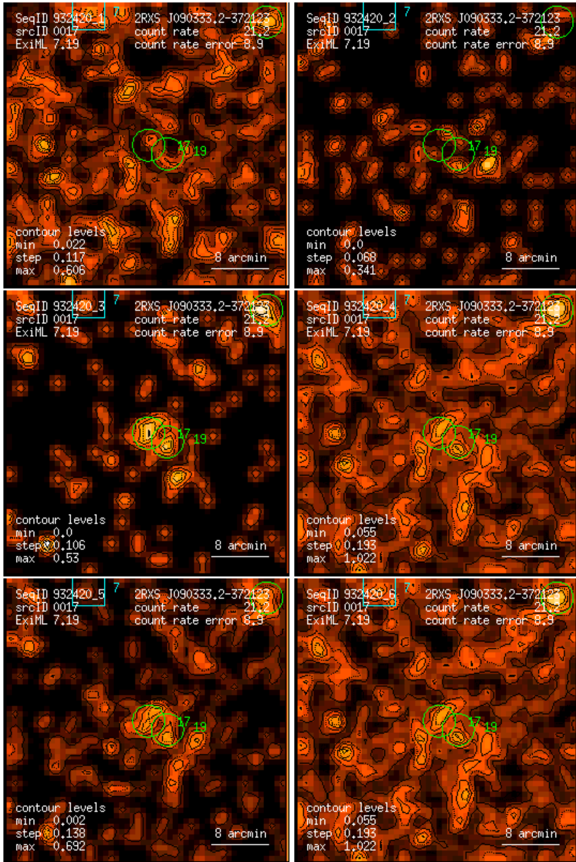
Figure 17: RASS 932420: detection 0017: band rate images, Gaussian filter: (1) PSPC channels 11 – 41, (2) 52 – 90, (3) 91 – 201, (4) 11 – 235, (5) 52 – 201, (6) 11 – 201. Broad band rates in counts/ks. Band rate contour levels in counts/ks/arcmin 2 .
