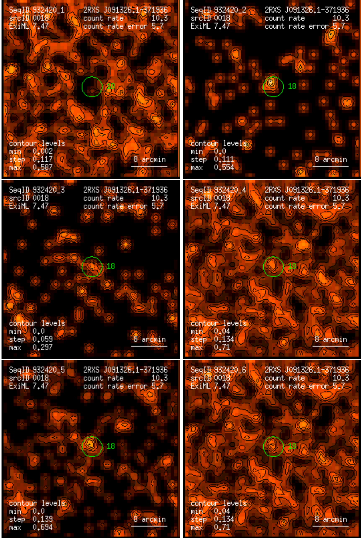
Figure 18: RASS 932420: detection 0018: band rate images, Gaussian filter: (1) PSPC channels 11 – 41, (2) 52 – 90, (3) 91 – 201, (4) 11 – 235, (5) 52 – 201, (6) 11 – 201. Broad band rates in counts/ks. Band rate contour levels in counts/ks/arcmin 2 .
