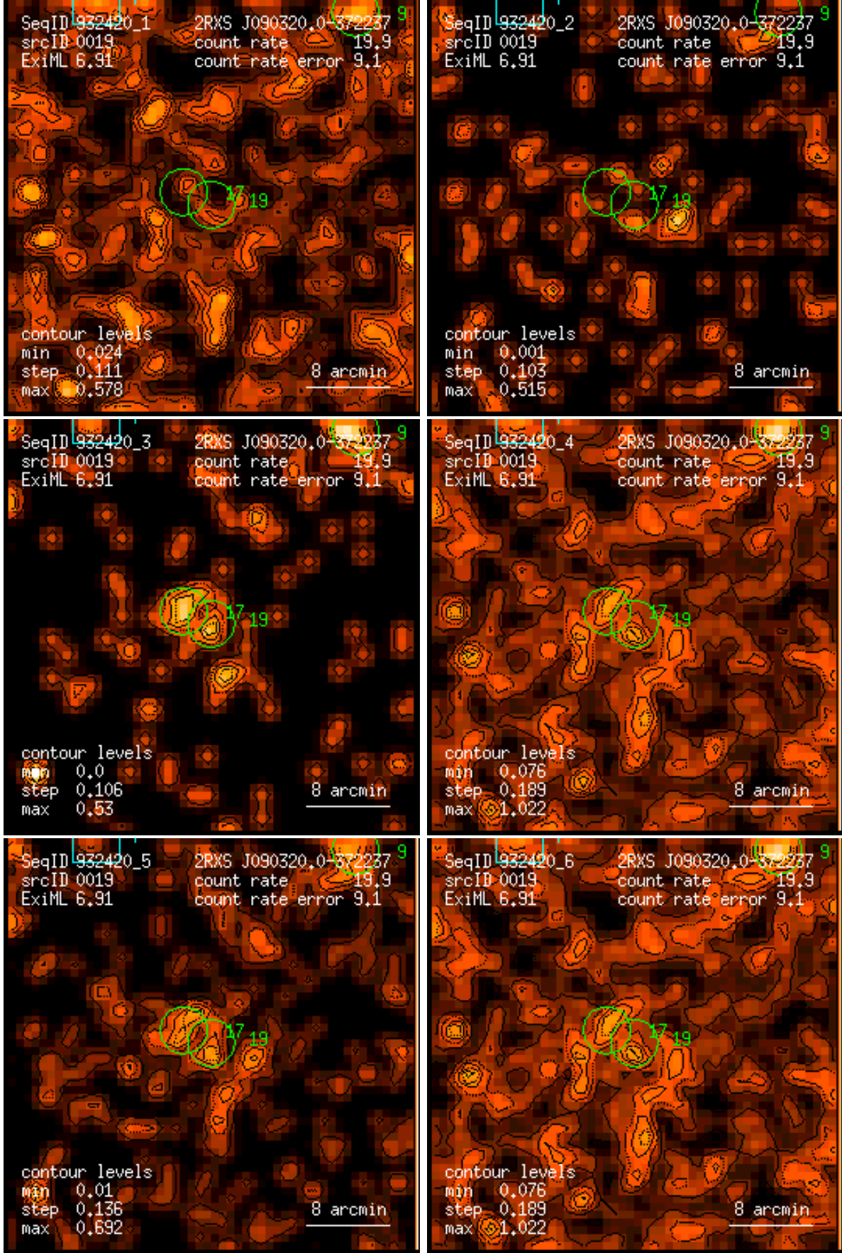
Figure 19: RASS 932420: detection 0019: band rate images, Gaussian filter: (1) PSPC channels 11 – 41, (2) 52 – 90, (3) 91 – 201, (4) 11 – 235, (5) 52 – 201, (6) 11 – 201. Broad band rates in counts/ks. Band rate contour levels in counts/ks/arcmin 2 .
