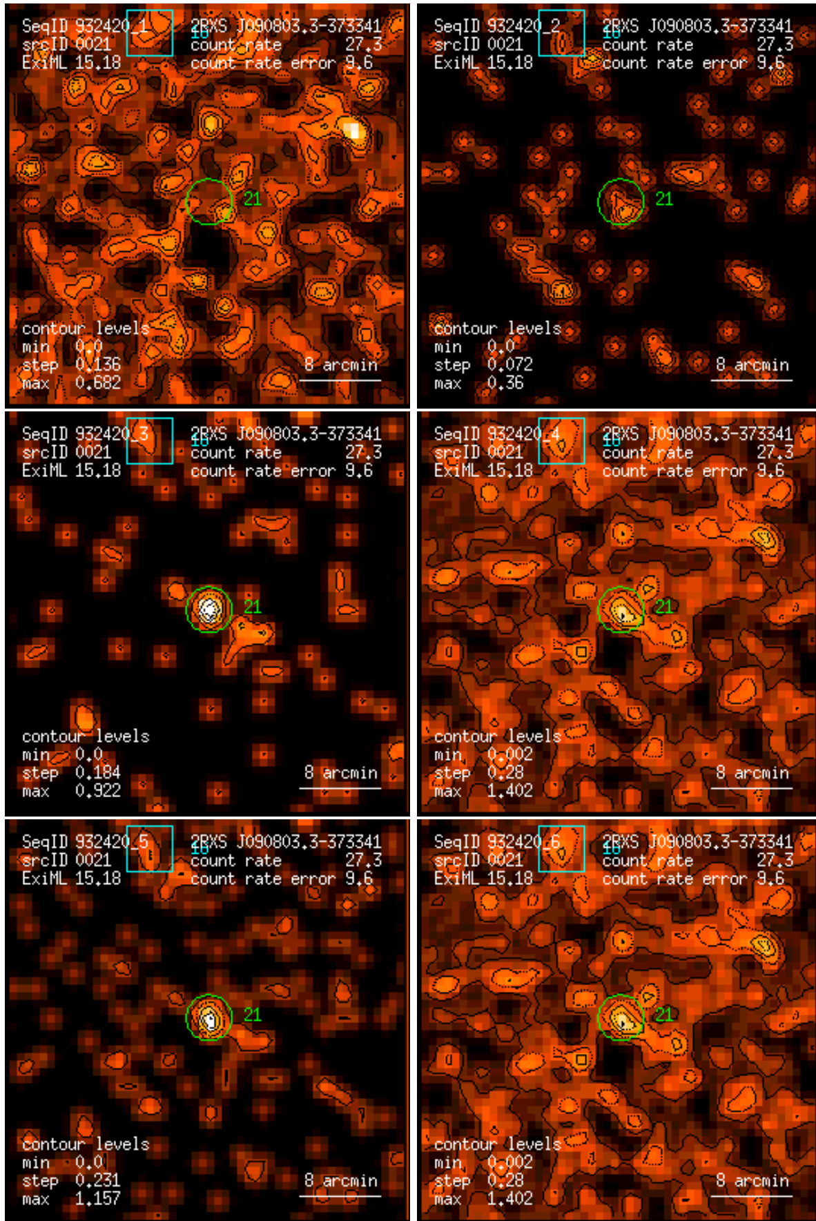
Figure 21: RASS 932420: detection 0021: band rate images, Gaussian filter: (1) PSPC channels 11 – 41, (2) 52 – 90, (3) 91 – 201, (4) 11 – 235, (5) 52 – 201, (6) 11 – 201. Broad band rates in counts/ks. Band rate contour levels in counts/ks/arcmin 2 .
