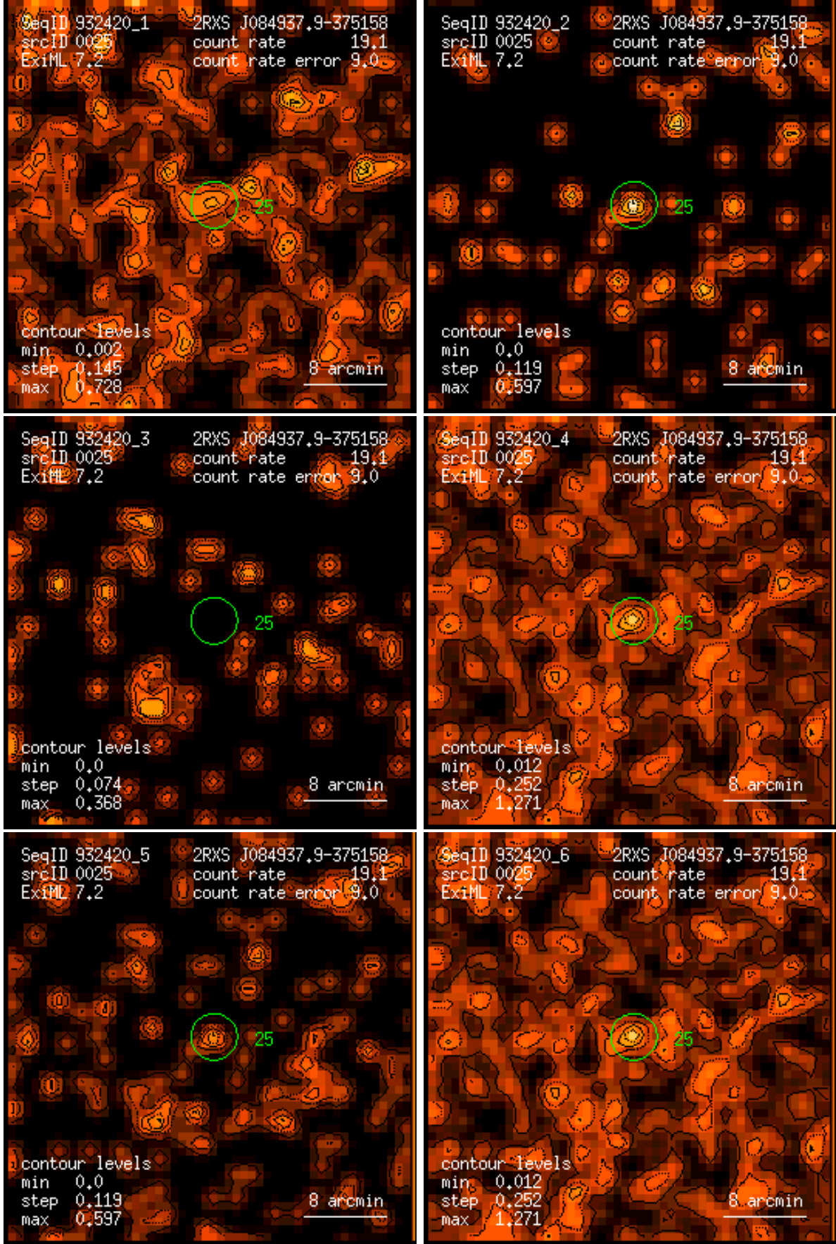
Figure 25: RASS 932420: detection 0025: band rate images, Gaussian filter: (1) PSPC channels 11 – 41, (2) 52 – 90, (3) 91 – 201, (4) 11 – 235, (5) 52 – 201, (6) 11 – 201. Broad band rates in counts/ks. Band rate contour levels in counts/ks/arcmin 2 .
