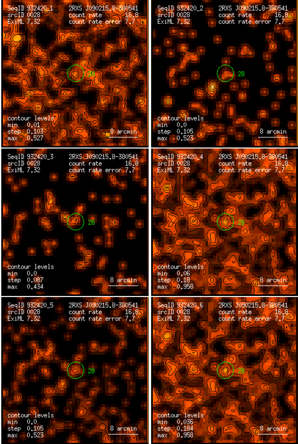
Figure 28: RASS 932420: detection 0028: band rate images, Gaussian filter: (1) PSPC channels 11 – 41, (2) 52 – 90, (3) 91 – 201, (4) 11 – 235, (5) 52 – 201, (6) 11 – 201. Broad band rates in counts/ks. Band rate contour levels in counts/ks/arcmin 2 .
