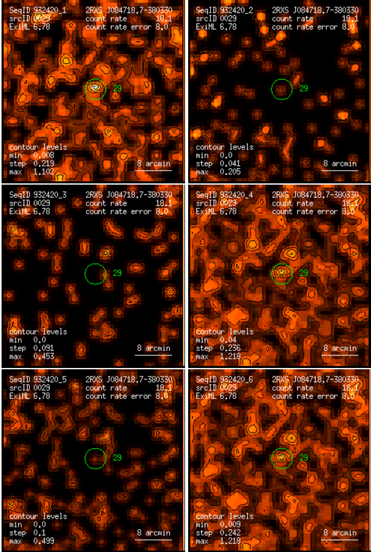
Figure 29: RASS 932420: detection 0029: band rate images, Gaussian filter: (1) PSPC channels 11 – 41, (2) 52 – 90, (3) 91 – 201, (4) 11 – 235, (5) 52 – 201, (6) 11 – 201. Broad band rates in counts/ks. Band rate contour levels in counts/ks/arcmin 2 .
