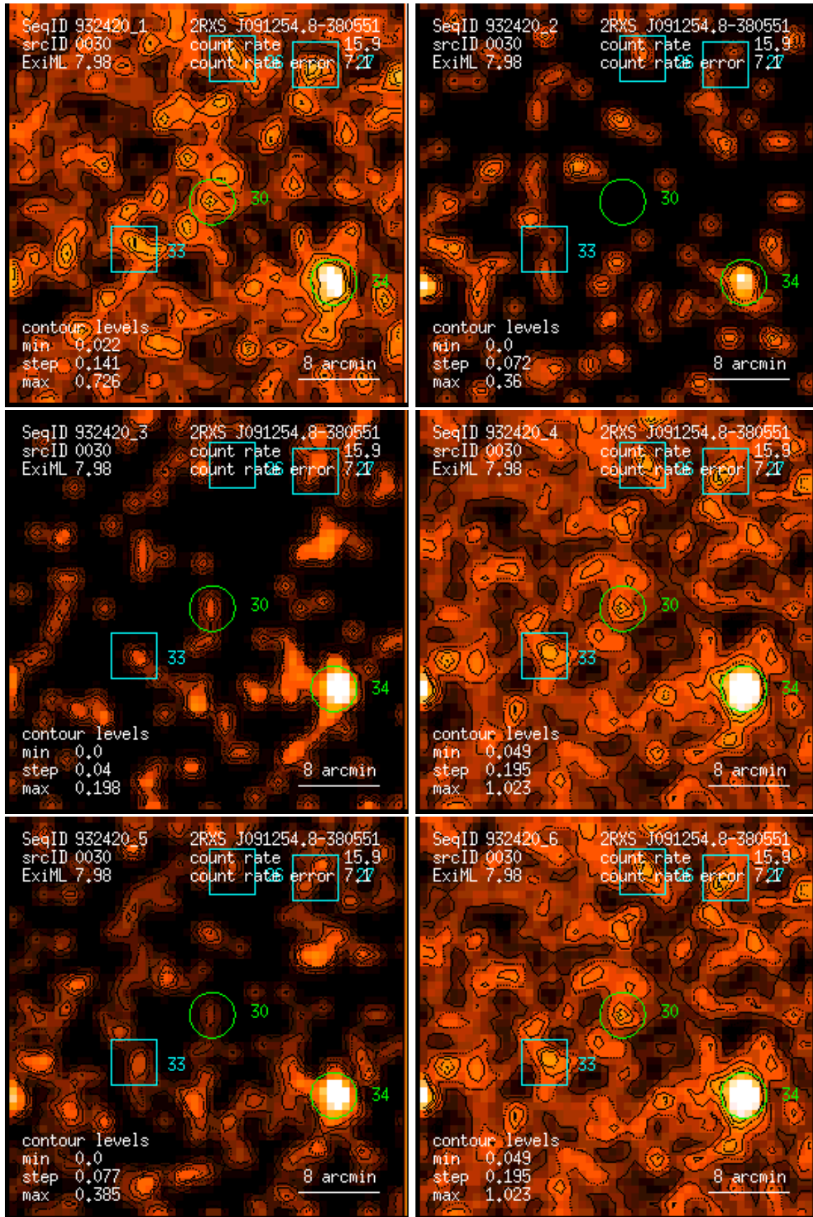
Figure 30: RASS 932420: detection 0030: band rate images, Gaussian filter: (1) PSPC channels 11 – 41, (2) 52 – 90, (3) 91 – 201, (4) 11 – 235, (5) 52 – 201, (6) 11 – 201. Broad band rates in counts/ks. Band rate contour levels in counts/ks/arcmin 2 .
