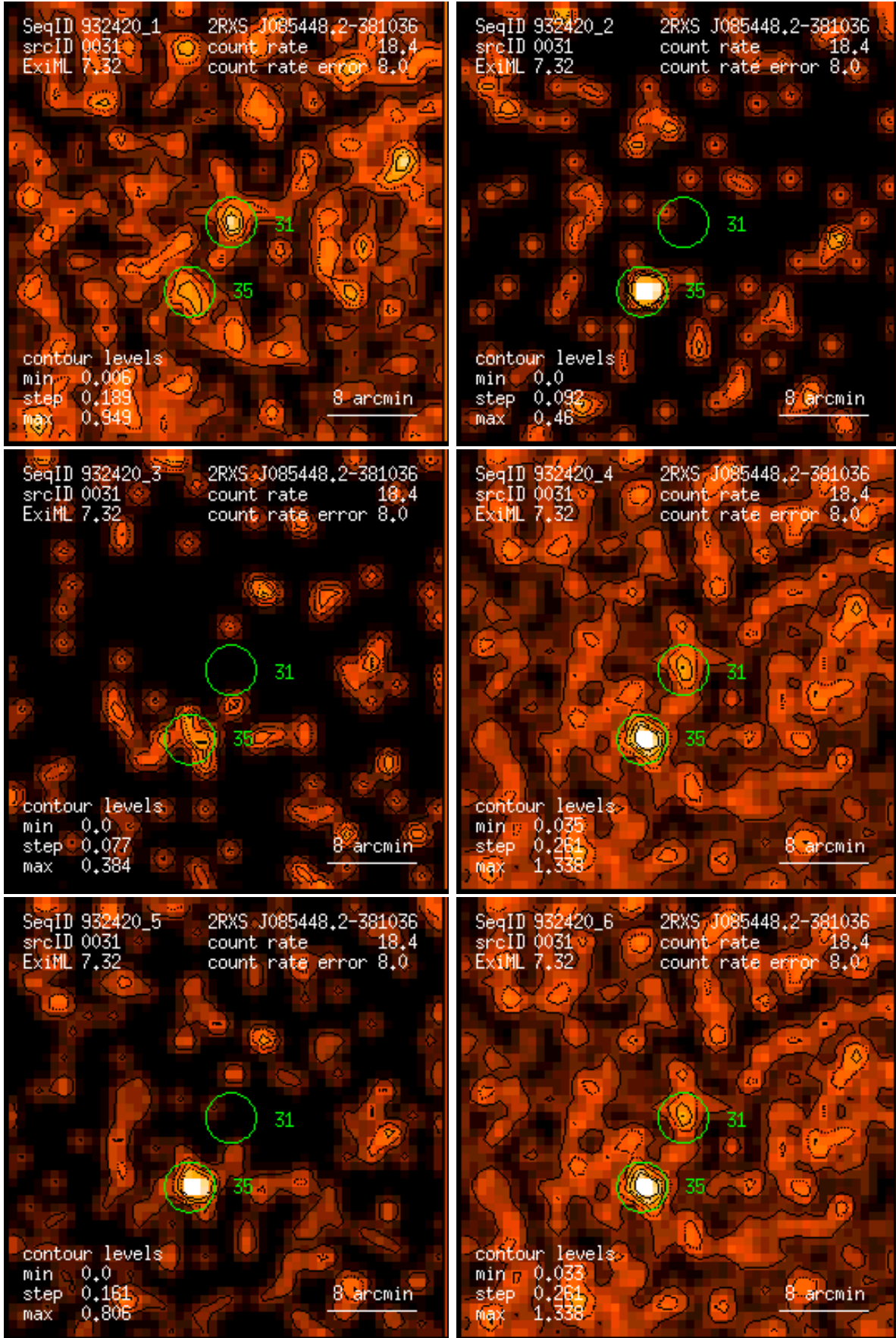
Figure 31: RASS 932420: detection 0031: band rate images, Gaussian filter: (1) PSPC channels 11 – 41, (2) 52 – 90, (3) 91 – 201, (4) 11 – 235, (5) 52 – 201, (6) 11 – 201. Broad band rates in counts/ks. Band rate contour levels in counts/ks/arcmin 2 .
