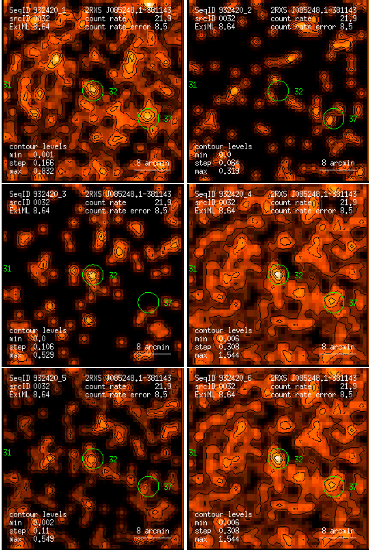
Figure 32: RASS 932420: detection 0032: band rate images, Gaussian filter: (1) PSPC channels 11 – 41, (2) 52 – 90, (3) 91 – 201, (4) 11 – 235, (5) 52 – 201, (6) 11 – 201. Broad band rates in counts/ks. Band rate contour levels in counts/ks/arcmin 2 .
