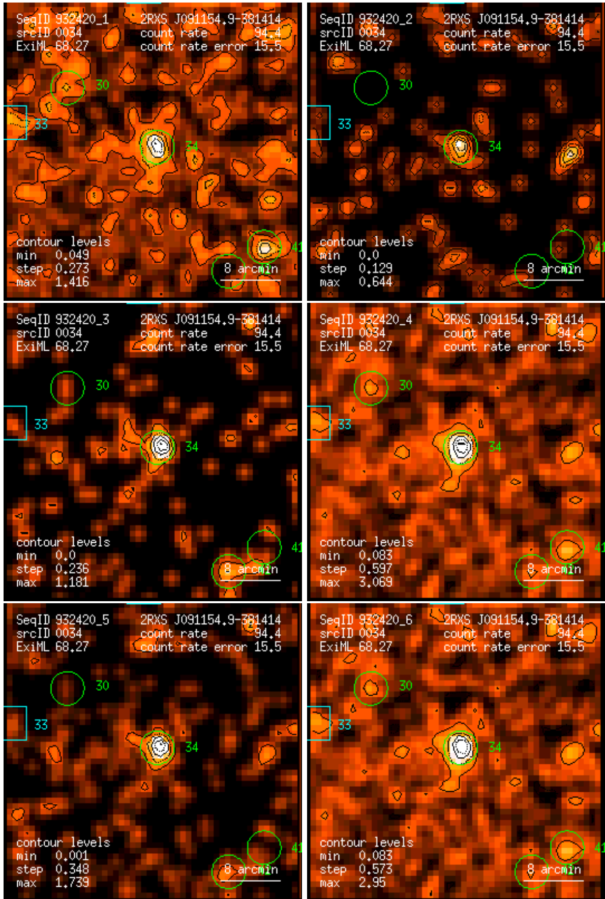
Figure 34: RASS 932420: detection 0034: band rate images, Gaussian filter: (1) PSPC channels 11 – 41, (2) 52 – 90, (3) 91 – 201, (4) 11 – 235, (5) 52 – 201, (6) 11 – 201. Broad band rates in counts/ks. Band rate contour levels in counts/ks/arcmin 2 .
