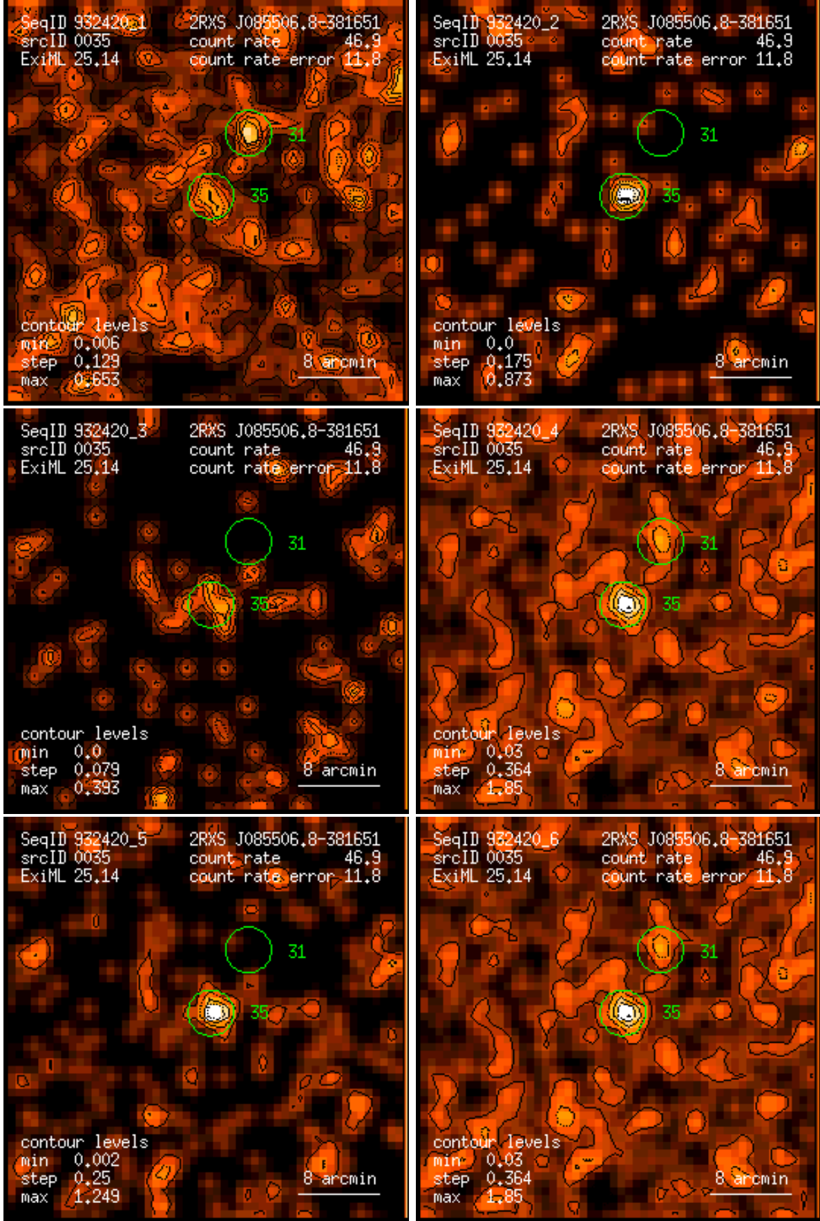
Figure 35: RASS 932420: detection 0035: band rate images, Gaussian filter: (1) PSPC channels 11 – 41, (2) 52 – 90, (3) 91 – 201, (4) 11 – 235, (5) 52 – 201, (6) 11 – 201. Broad band rates in counts/ks. Band rate contour levels in counts/ks/arcmin 2 .
